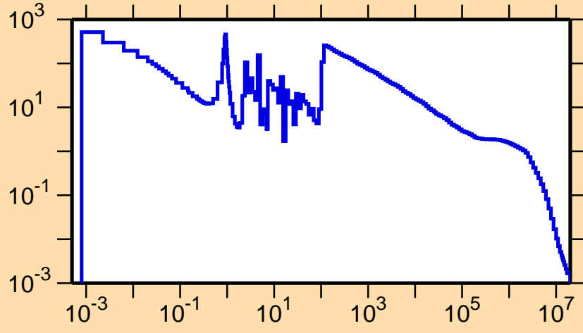
\sigma vs. E for ^{155}\text{Yb}(n,\gamma)
