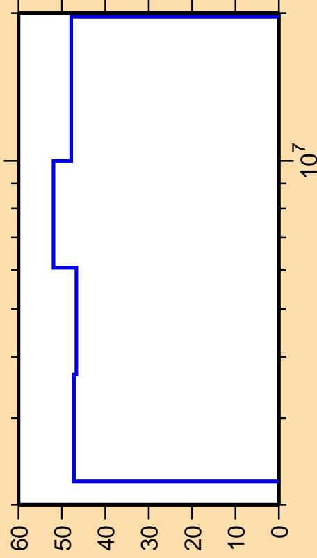
\Delta\sigma/\sigma vs. E for ^{155}\text{Yb}(n,ncont.)
