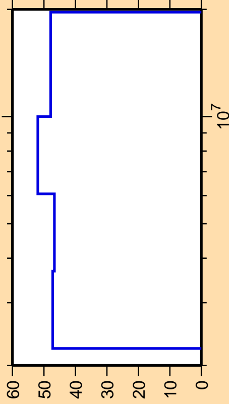
\Delta\sigma/\sigma vs. E for ^{155}\text{Yb}(n,n\text{cont.})
