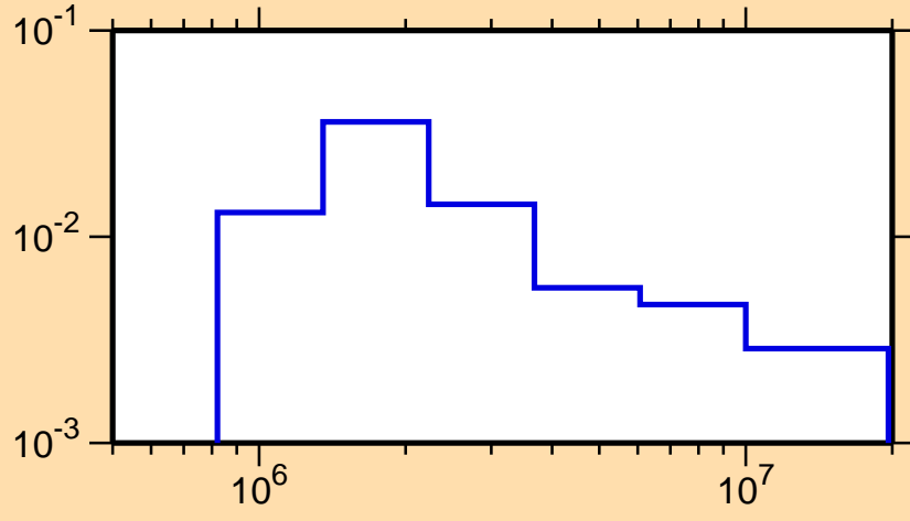
\sigma vs. E for ^{155}\text{Yb}(n,n_2)
