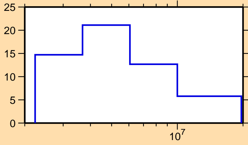
\Delta\sigma/\sigma vs. E for ^{155}\text{Yb}(n,el.)
