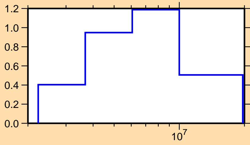
\sigma vs. E for ^{155}\text{Yb}(n,n\text{cont.})
