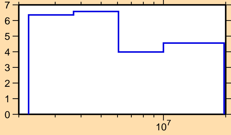
\Delta\sigma/\sigma vs. E for ^{155}\text{Yb}(n,n_{\text{nonel.}})
