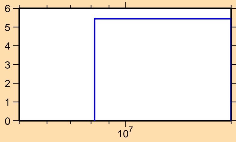
\Delta\sigma/\sigma vs. E for ^{155}\text{Yb}(n,\text{el.})
