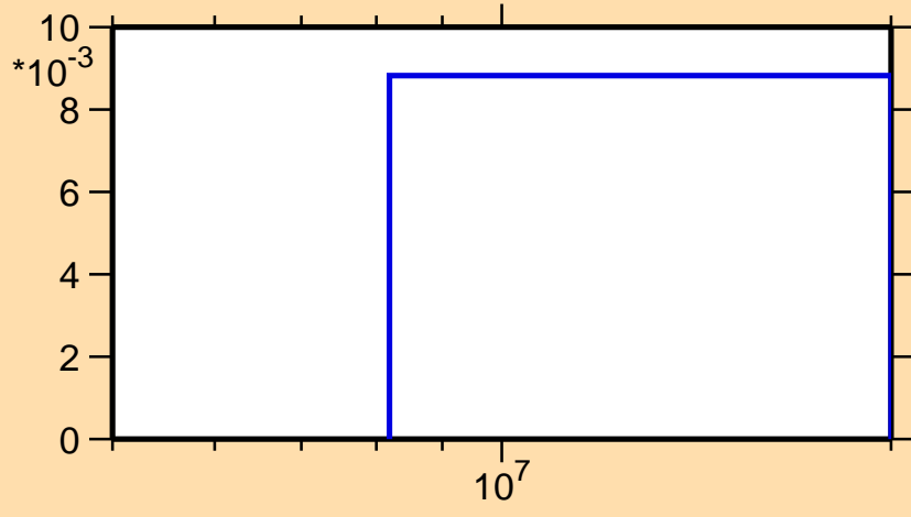
\sigma vs. E for ^{155}\text{Yb}(n,2n\alpha)
