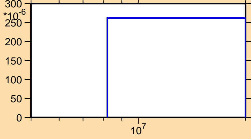
\sigma vs. E for ^{155}\text{Yb}(n,2np)
