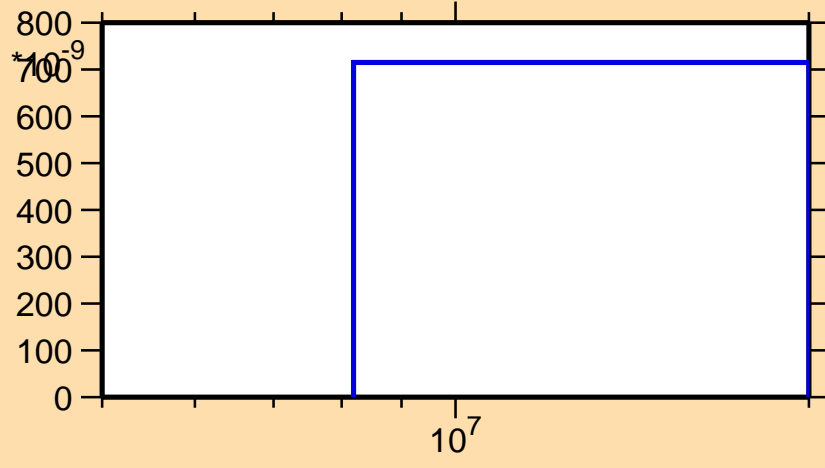
\sigma vs. E for ^{155}\text{Yb}(n,\text{pt})
