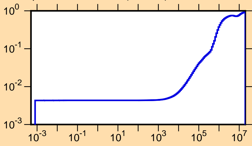
\mu vs. E for ^{156}\text{Yb}(\text{mt251})
