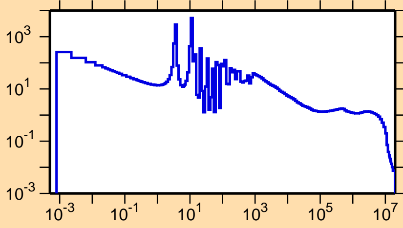
\sigma vs. E for ^{156}\text{Yb}(n,\gamma)
