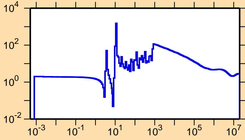
\sigma vs. E for ^{156}\text{Yb}(n,\text{el.})
