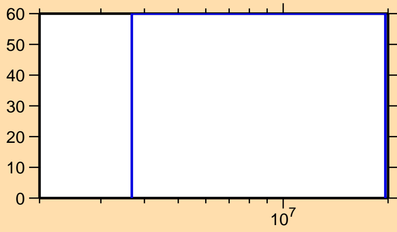
\Delta\sigma/\sigma vs. E for ^{156}\text{Yb}(n,n_1)
