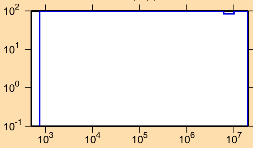
\Delta\sigma/\sigma vs. E for ^{156}\text{Yb}(n,p)
