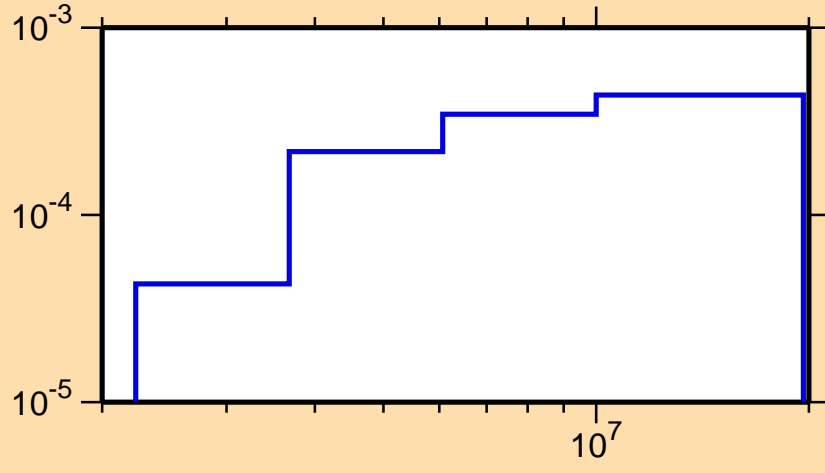
\sigma vs. E for ^{156}\text{Yb}(n,n_4)
