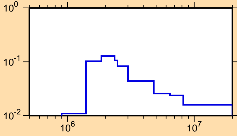
\sigma vs. E for ^{156}\text{Yb}(n,n_2)
