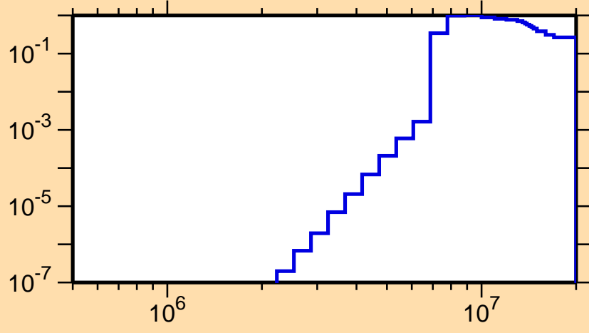
\sigma vs. E for ^{157}\text{Yb}(n,n\alpha)
