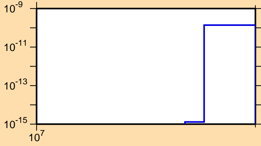
\sigma vs. E for ^{157}\text{Yb}(n,nt)
