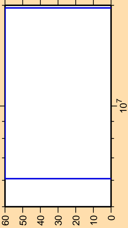
\Delta\sigma/\sigma vs. E for ^{157}\text{Yb}(n,2n)
