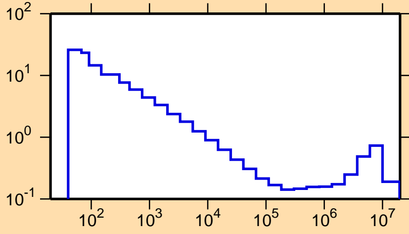
\sigma vs. E for ^{157}\text{Yb}(n,p)
