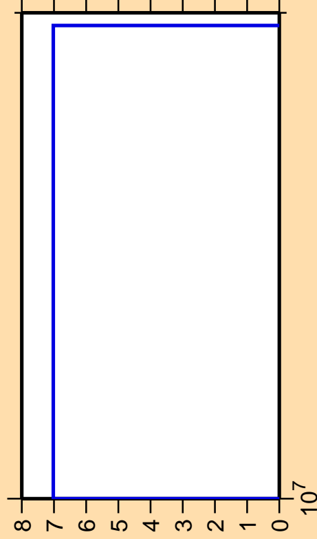
\Delta\sigma/\sigma vs. E for ^{157}\text{Yb}(n,nt)
