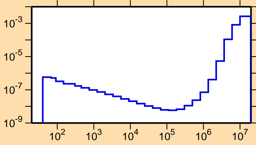
\sigma vs. E for ^{157}\text{Yb}(n,p\alpha)
