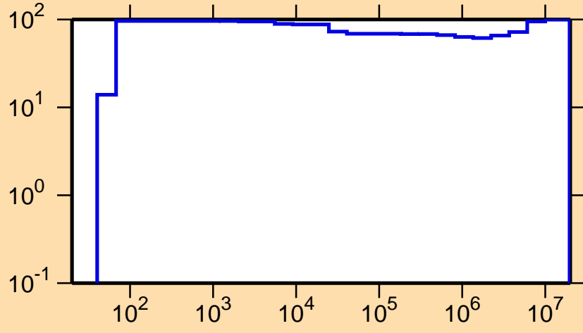
\Delta\sigma/\sigma vs. E for ^{157}\text{Yb}(n,\gamma)
