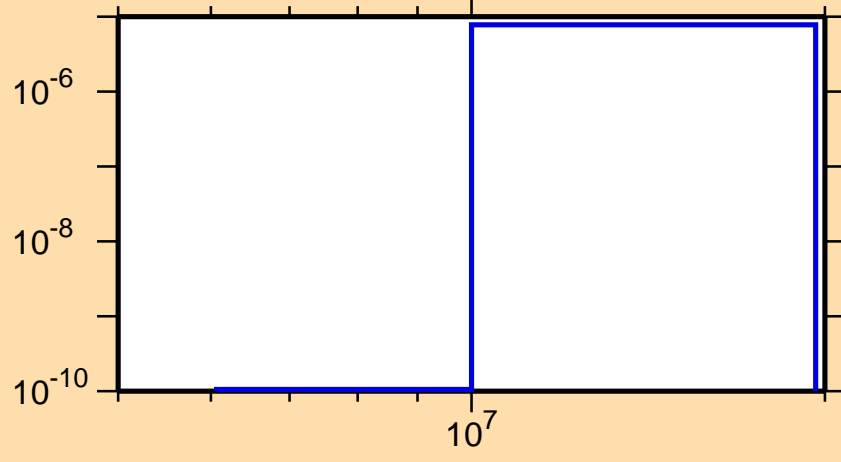
\sigma vs. E for ^{157}\text{Yb}(n,\text{He3})
