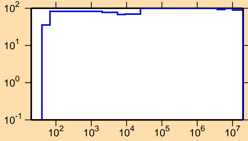
\Delta\sigma/\sigma vs. E for ^{157}\text{Yb}(n,p)
