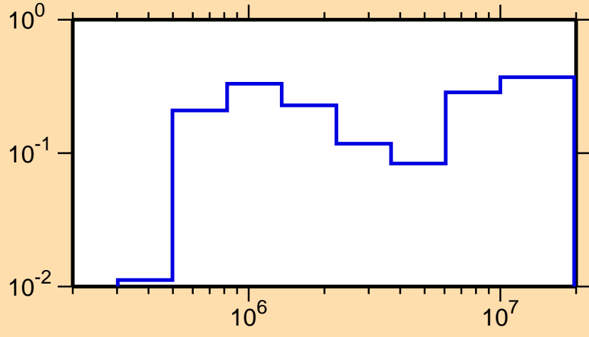
\sigma vs. E for ^{157}\text{Yb}(n,\text{inel.})
