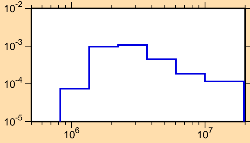
\sigma vs. E for ^{157}\text{Yb}(n,n_4)
