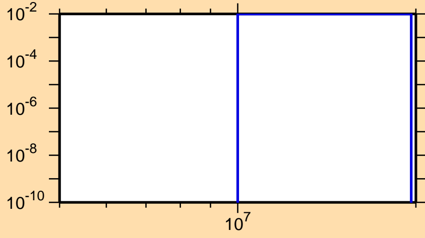
\sigma vs. E for ^{157}\text{Yb}(n,2n\alpha)
