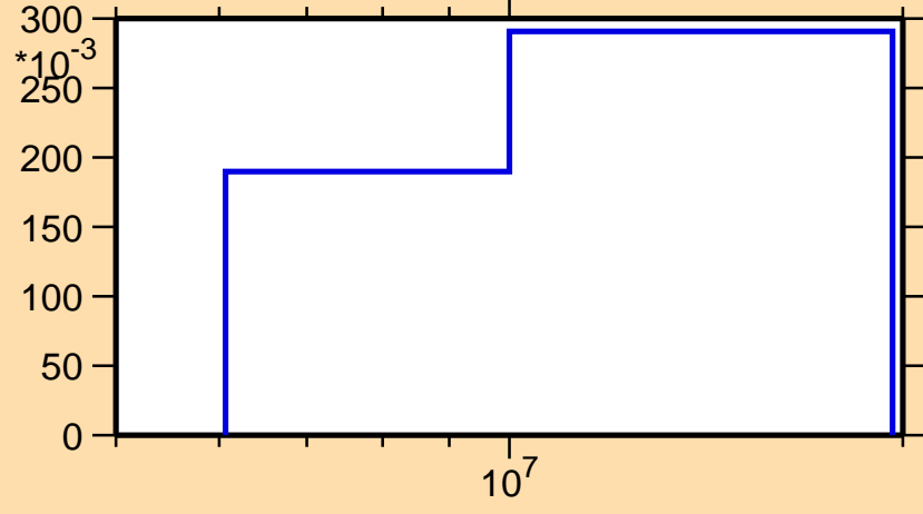
\sigma vs. E for ^{157}\text{Yb}(n,n\text{cont.})
