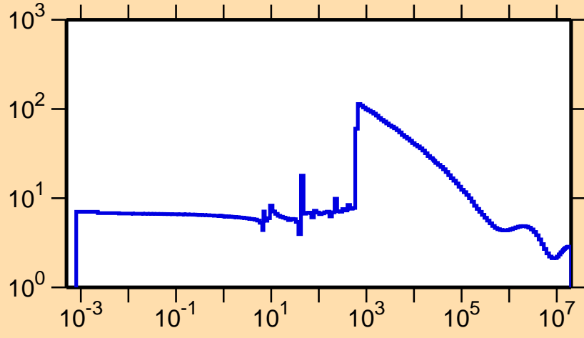
\sigma vs. E for ^{158}\text{Yb}(n,\text{el.})
