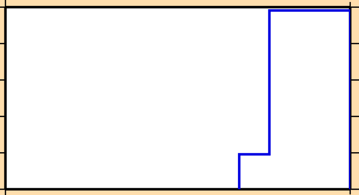
\sigma vs. E for ^{158}\text{Yb}(n,2np)
