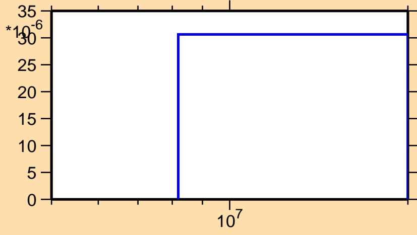
\sigma vs. E for ^{158}\text{Yb}(n,t)
