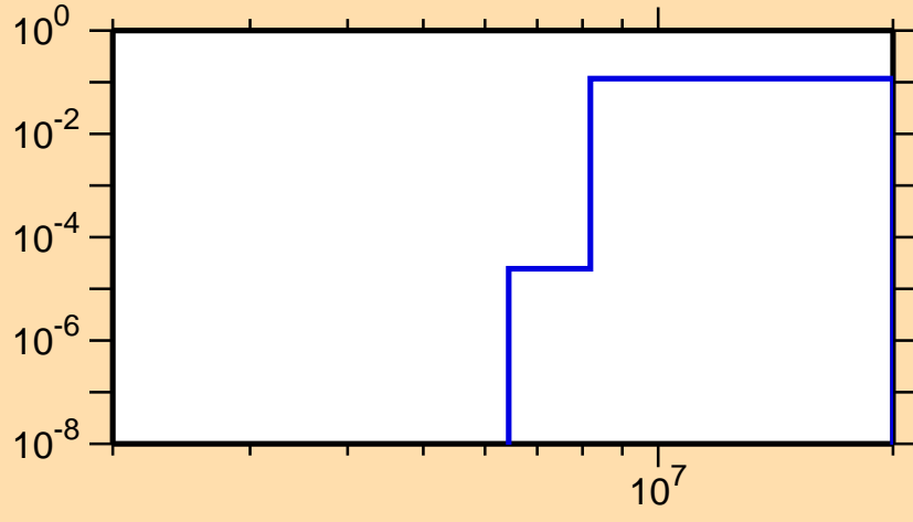
\sigma vs. E for ^{158}\text{Yb}(n,np)
