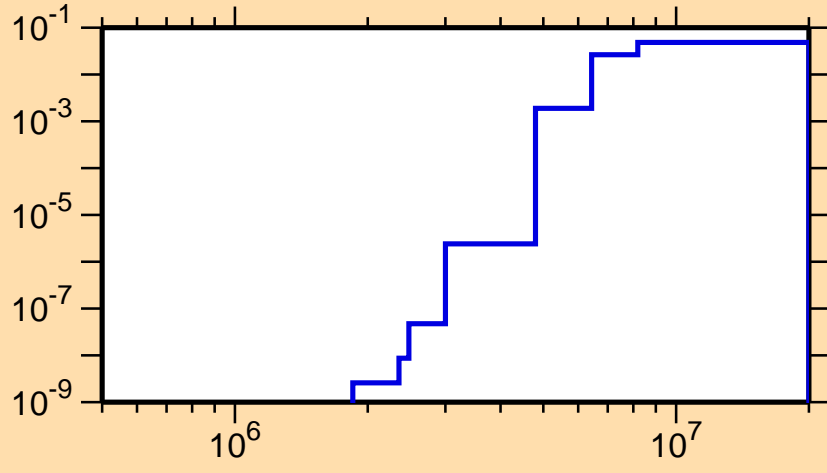
\sigma vs. E for ^{158}\text{Yb}(n,n\alpha)
