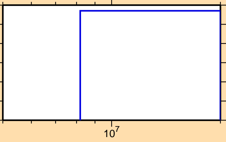
\sigma vs. E for ^{158}\text{Yb}(\text{mt117})
