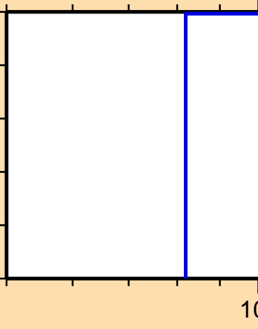
\sigma vs. E for ^{159}\text{Yb}(n,\text{He}3)
