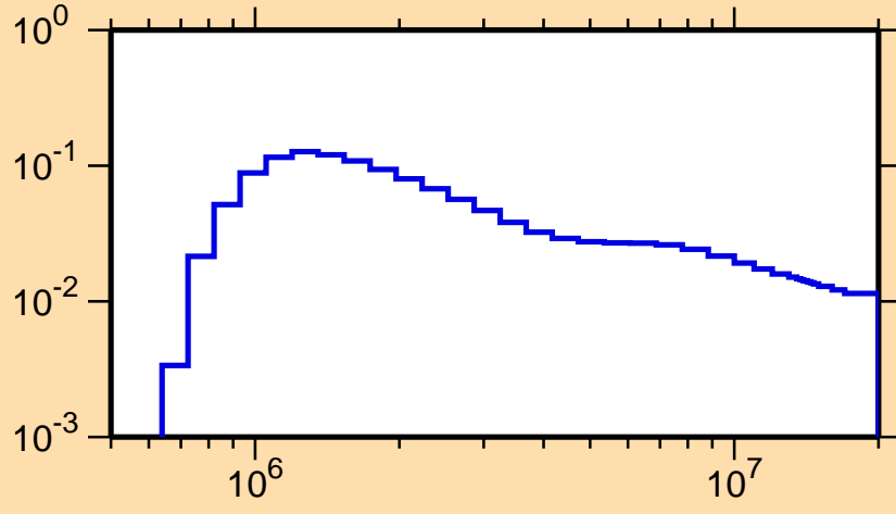
\sigma vs. E for ^{160}\text{Yb}(n,n_2)
