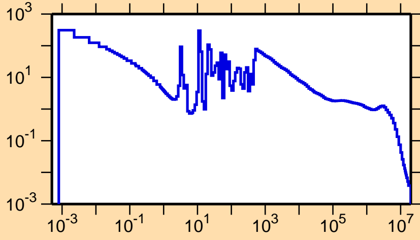
\sigma vs. E for ^{160}\text{Yb}(n,\gamma)
