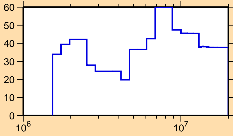
\Delta\sigma/\sigma vs. E for ^{160}\text{Yb}(n, el.)
