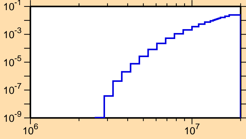
\sigma vs. E for ^{160}\text{Yb}(n,n\alpha)
