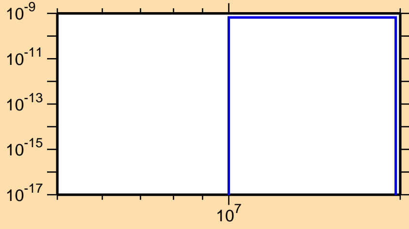
\sigma vs. E for ^{160}\text{Yb}(\text{mt117})
