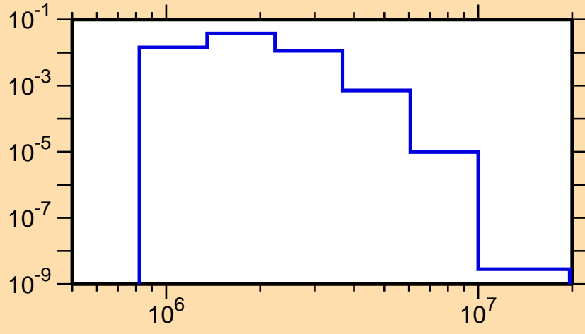
\sigma vs. E for ^{160}\text{Yb}(n,n_4)
