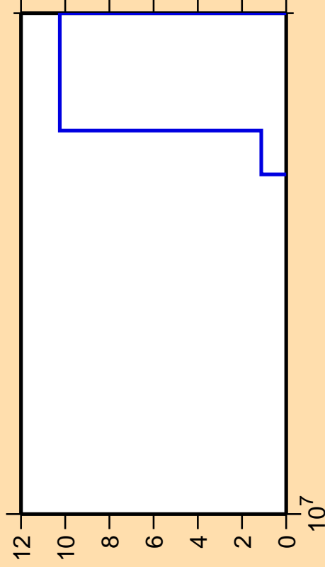
\Delta\sigma/\sigma vs. E for ^{161}\text{Yb}(n,3n\alpha)
