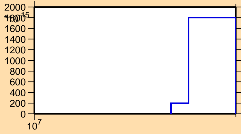
\sigma vs. E for ^{161}\text{Yb}(n,3n\alpha)
