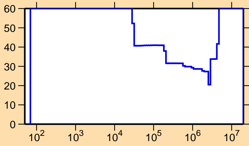
\Delta\sigma/\sigma vs. E for ^{161}\text{Yb}(n,\gamma)
