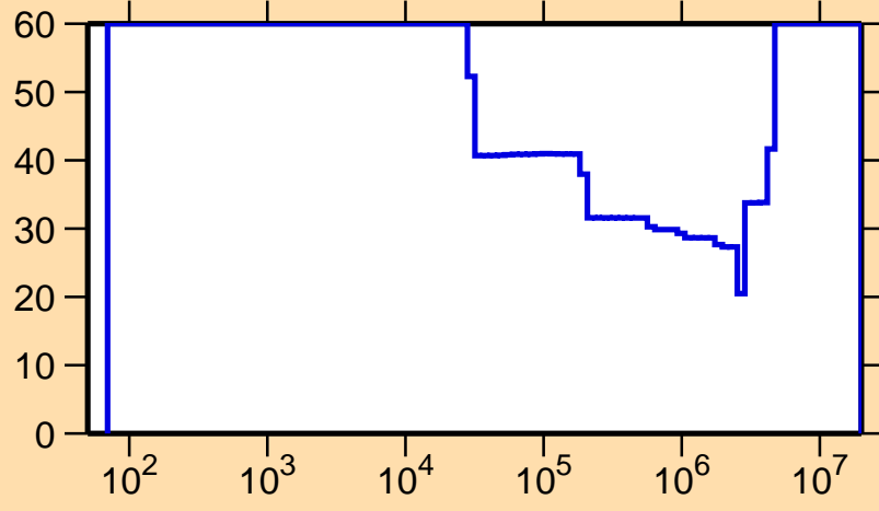
\Delta\sigma/\sigma vs. E for ^{161}\text{Yb}(n,\gamma)
