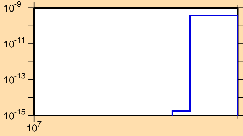
\sigma vs. E for ^{161}\text{Yb}(n,nt)
