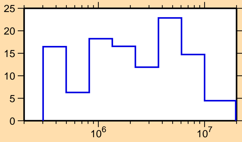
\Delta\sigma/\sigma vs. E for ^{161}\text{Yb}(n, el.)
