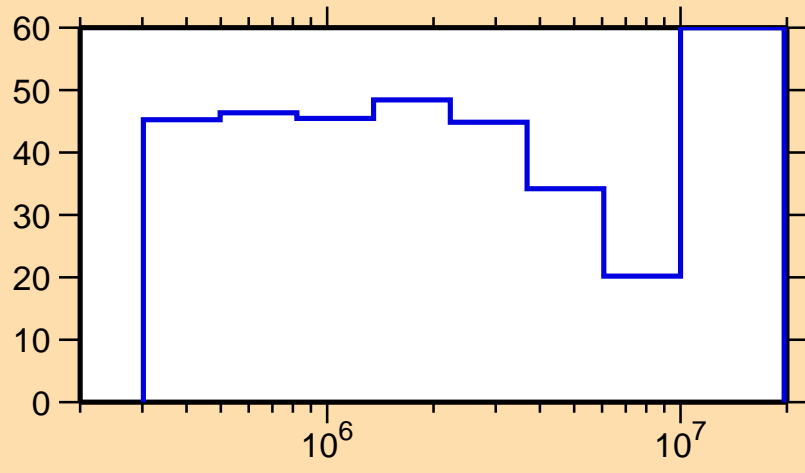
\Delta\sigma/\sigma vs. E for ^{161}\text{Yb}(n,n\text{cont.})
