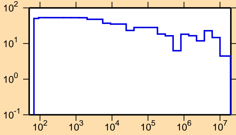
\Delta\sigma/\sigma vs. E for ^{161}\text{Yb}(n,el.)
