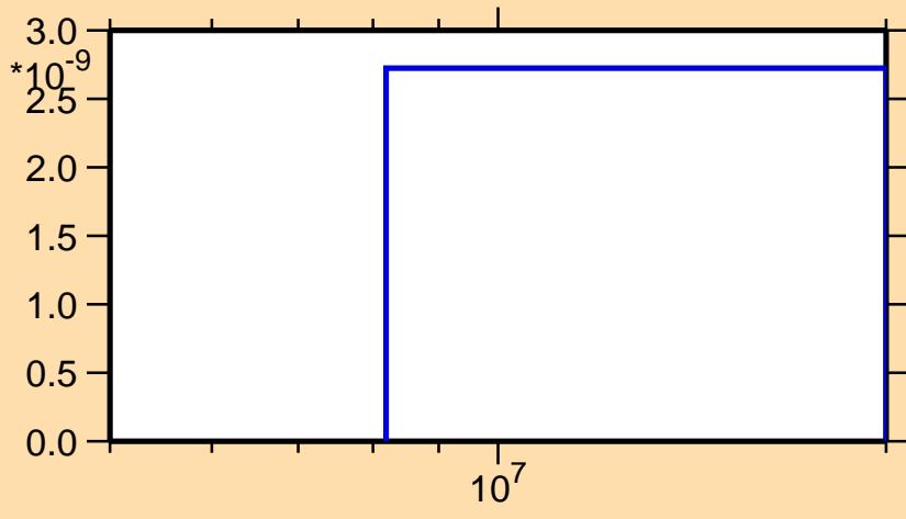
\sigma vs. E for ^{161}\text{Yb} (mt 45)
