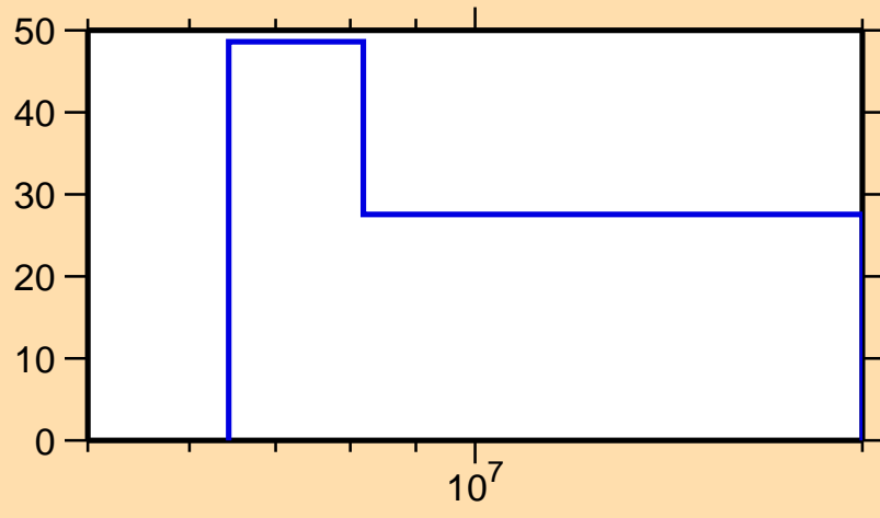
\Delta\sigma/\sigma vs. E for ^{161}\text{Yb}(n,2n)
