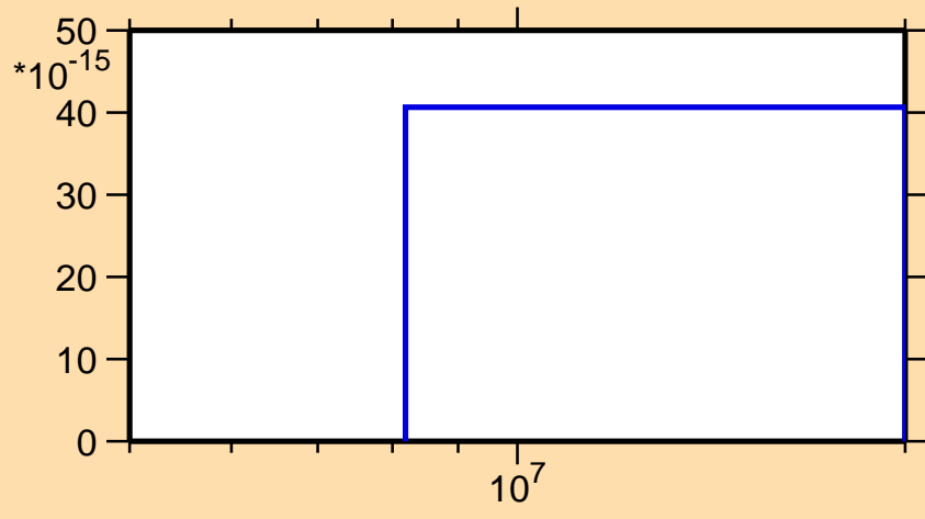
\sigma vs. E for ^{161}\text{Yb}(n,3n\alpha)
