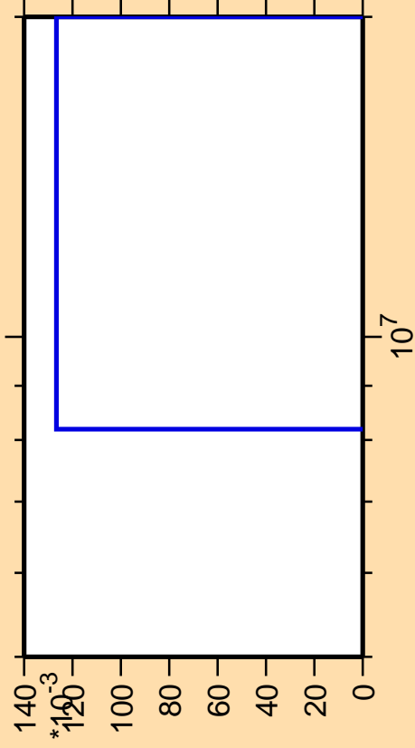
\Delta\sigma/\sigma vs. E for ^{161}\text{Yb}(n,3n\alpha)
