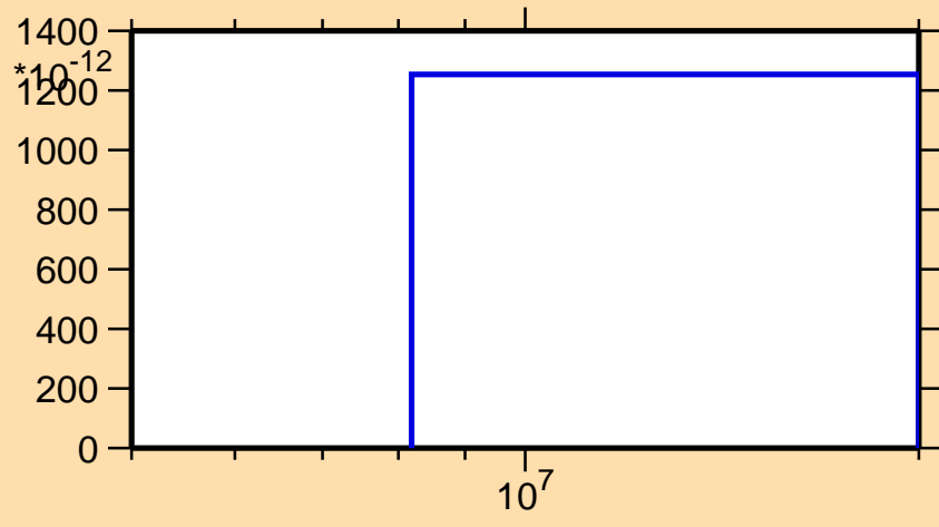
\sigma vs. E for ^{161}\text{Yb}(n,\text{pd})
