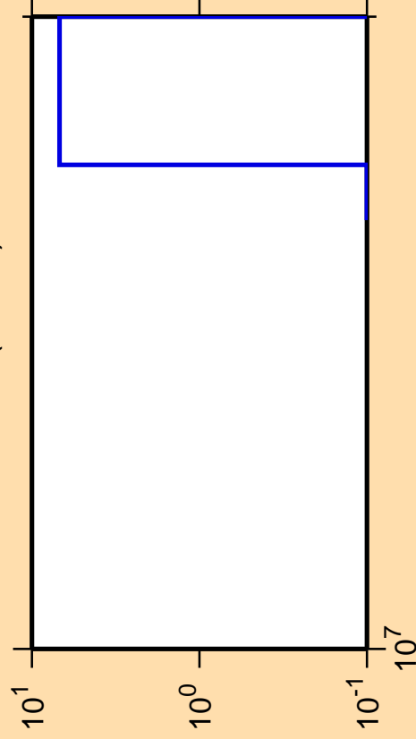
\Delta\sigma/\sigma vs. E for ^{162}\text{Yb} (mt 34)
