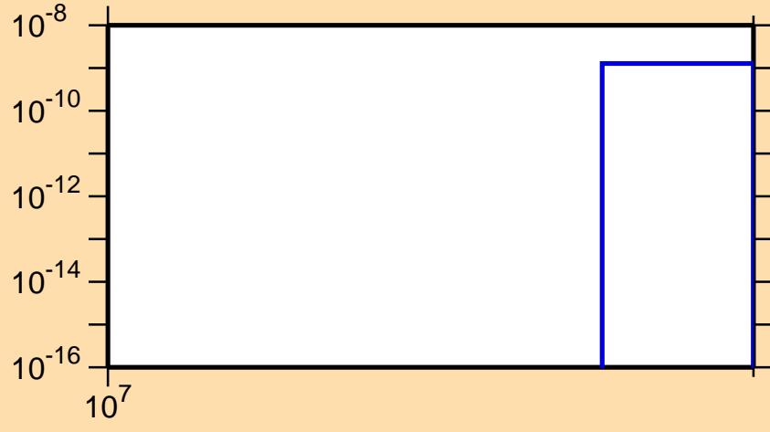
\sigma vs. E for ^{162}\text{Yb}(n,3n\alpha)
