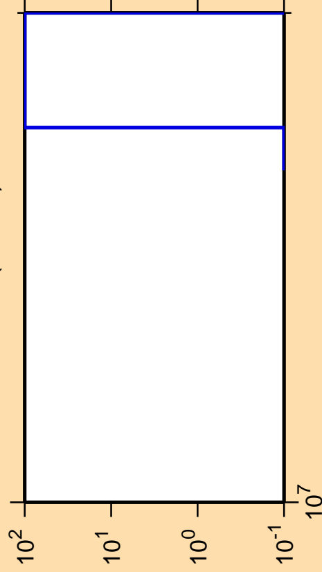
\Delta\sigma/\sigma vs. E for ^{162}\text{Yb}(n,3n\alpha)
