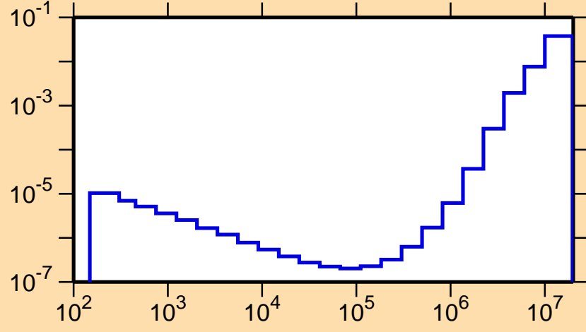
\sigma vs. E for ^{162}\text{Yb}(n,p)
