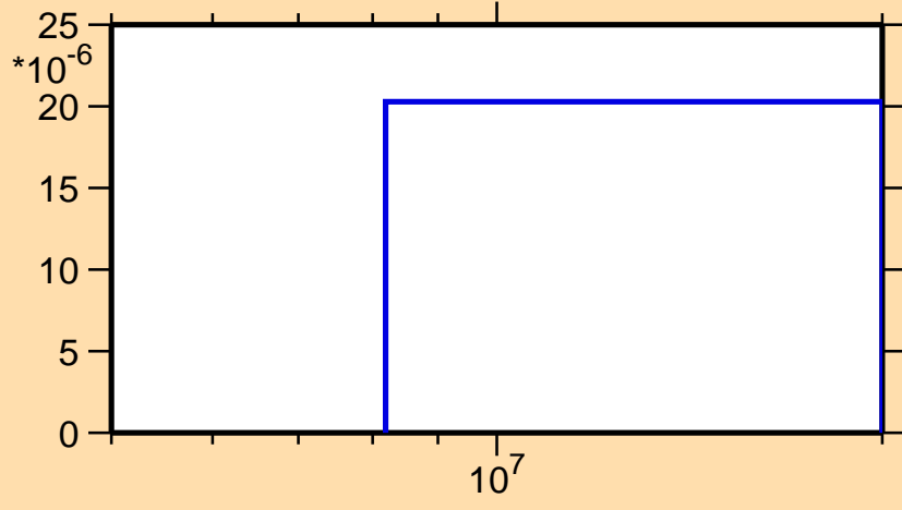
\sigma vs. E for ^{162}\text{Yb}(n,t)
