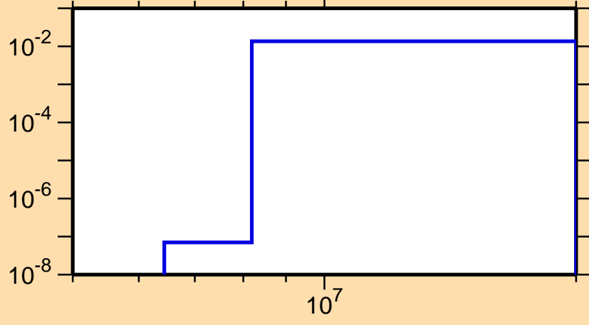
\sigma vs. E for ^{162}\text{Yb}(n,np)
