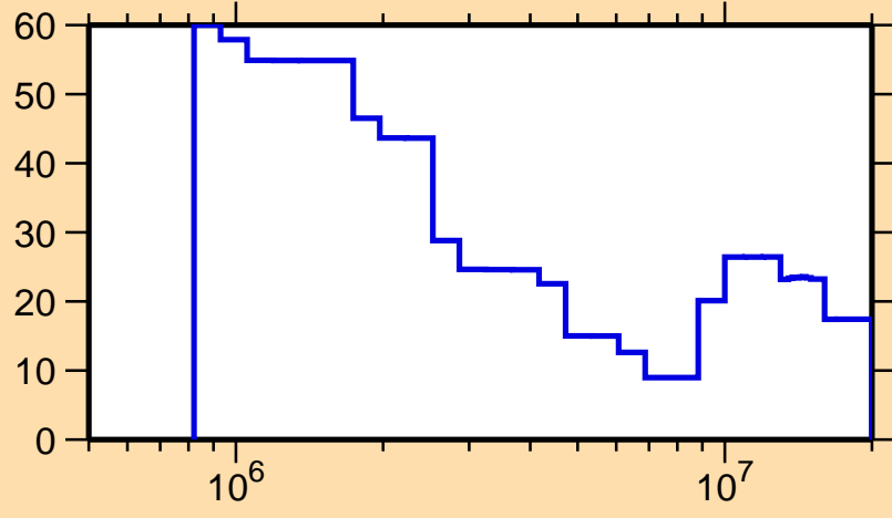
\Delta\sigma/\sigma vs. E for ^{163}\text{Yb}(n,n\text{cont.})
