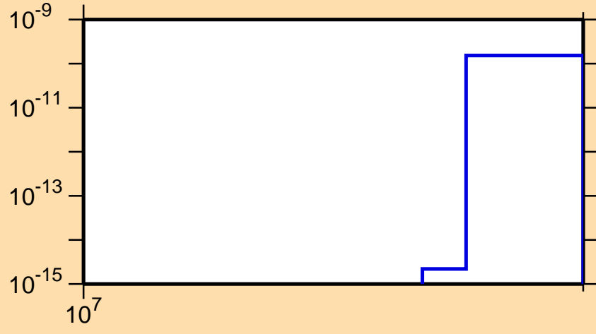
\sigma vs. E for ^{163}\text{Yb}(n,nt)
