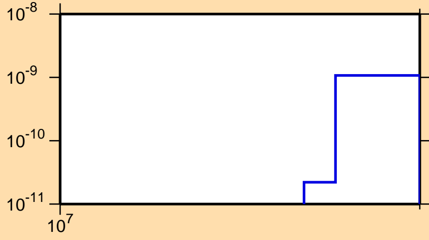
\sigma vs. E for ^{163}\text{Yb}(n,\text{pt})
