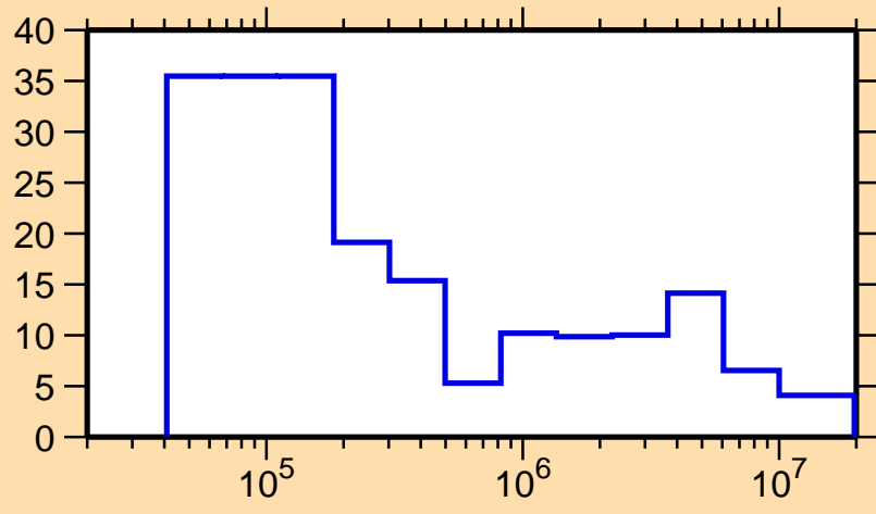
\Delta\sigma/\sigma vs. E for ^{163}\text{Yb}(n,\text{el.})
