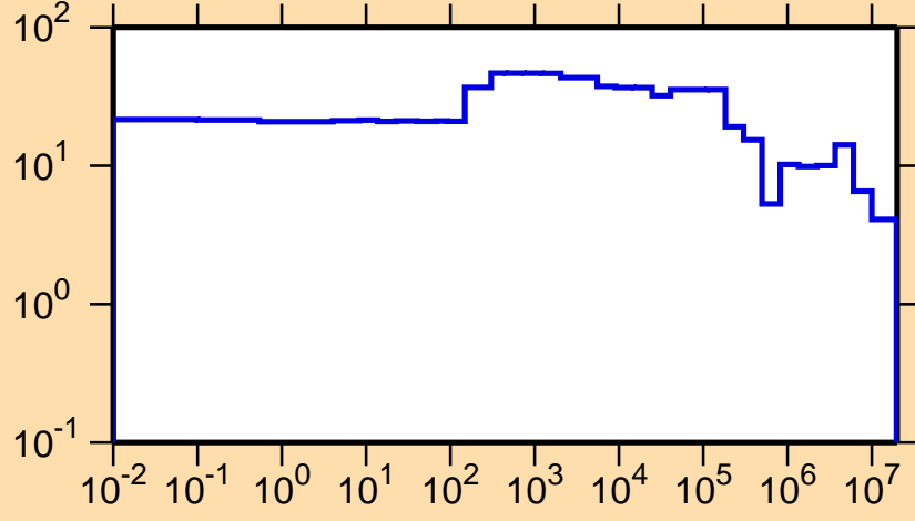
\Delta\sigma/\sigma vs. E for ^{163}\text{Yb}(n,\text{el.})
