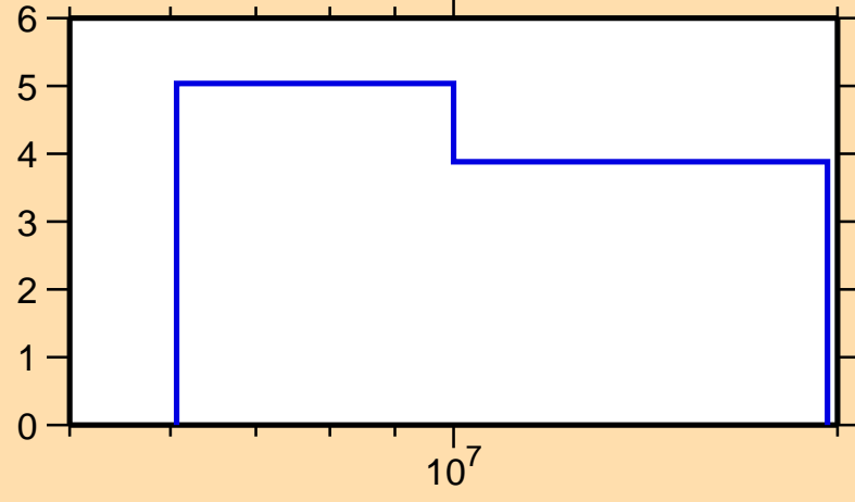
\Delta\sigma/\sigma vs. E for ^{163}\text{Yb}(n,\text{nonel.})
