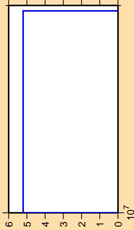
\Delta\sigma/\sigma vs. E for ^{163}\text{Yb}(n,nt)
