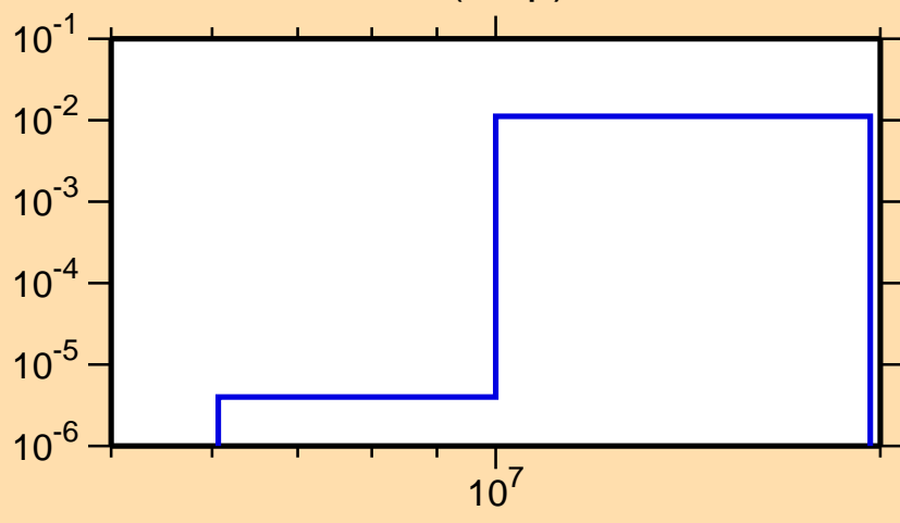
\sigma vs. E for ^{163}\text{Yb}(n,np)
