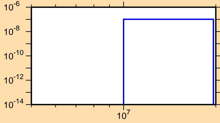
\sigma vs. E for ^{163}\text{Yb}(n,\text{He3})
