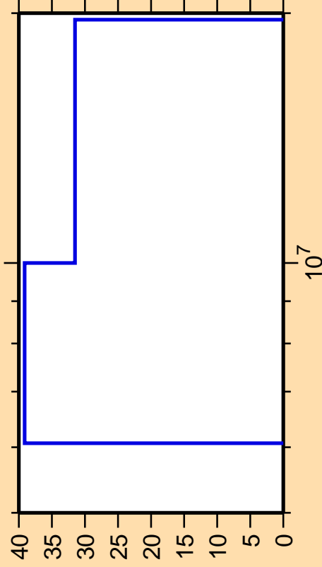
\Delta\sigma/\sigma vs. E for ^{163}\text{Yb}(n,n_1)
