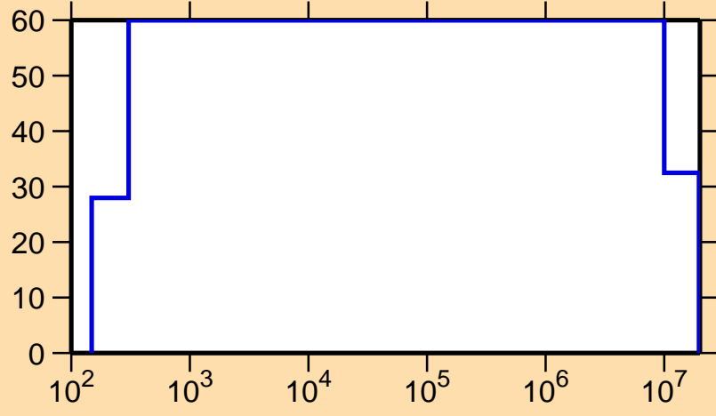
\Delta\sigma/\sigma vs. E for ^{163}\text{Yb}(n,p)
