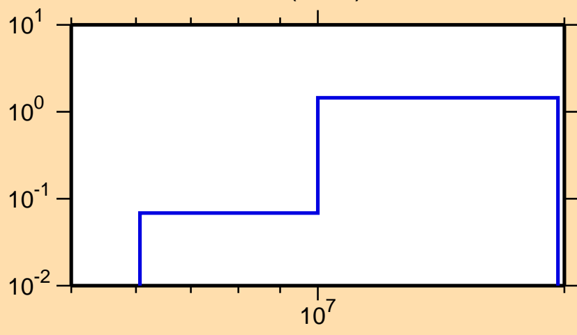
\sigma vs. E for ^{163}\text{Yb}(n,2n)
