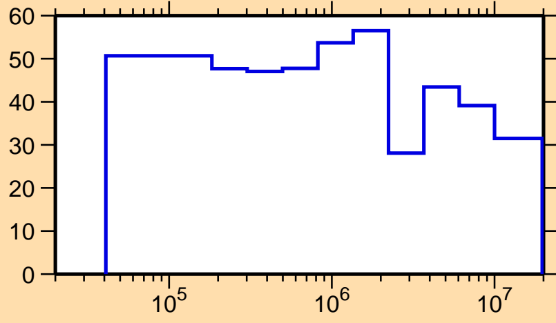
\Delta\sigma/\sigma vs. E for ^{163}\text{Yb}(n,n_1)
