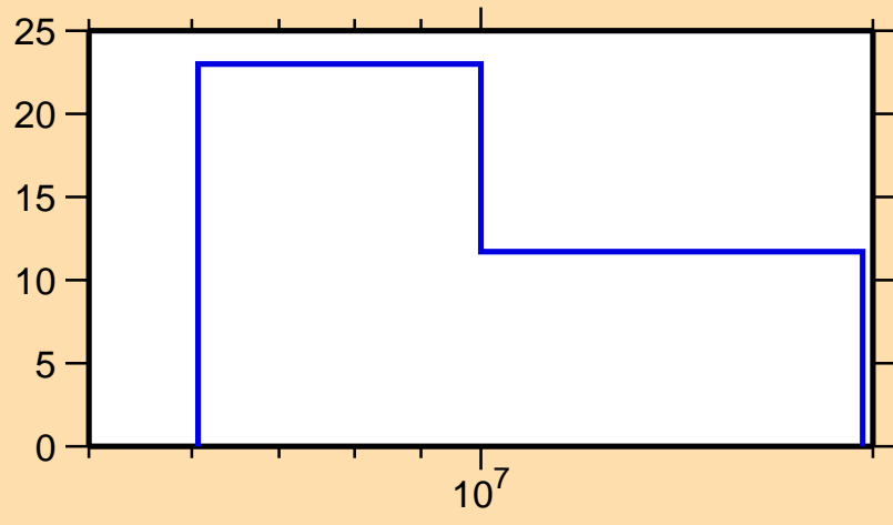
\Delta\sigma/\sigma vs. E for ^{163}\text{Yb}(n,2n)
