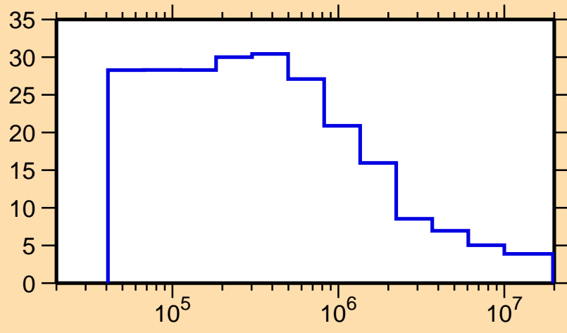
\Delta\sigma/\sigma vs. E for ^{163}\text{Yb}(n,\text{nonel.})
