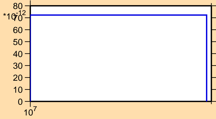
\sigma vs. E for ^{163}\text{Yb}(n,\text{pd})
