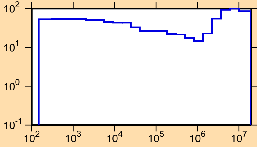
\Delta\sigma/\sigma vs. E for ^{163}\text{Yb}(n,\gamma)
