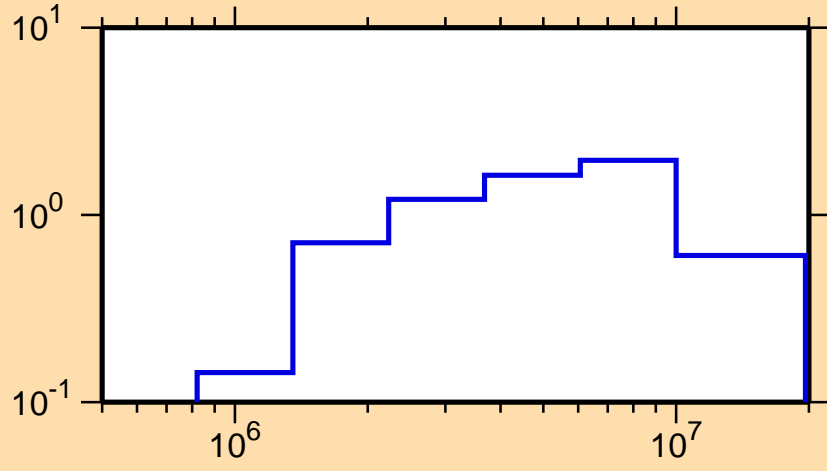
\sigma vs. E for ^{163}\text{Yb}(n,n\text{cont.})
