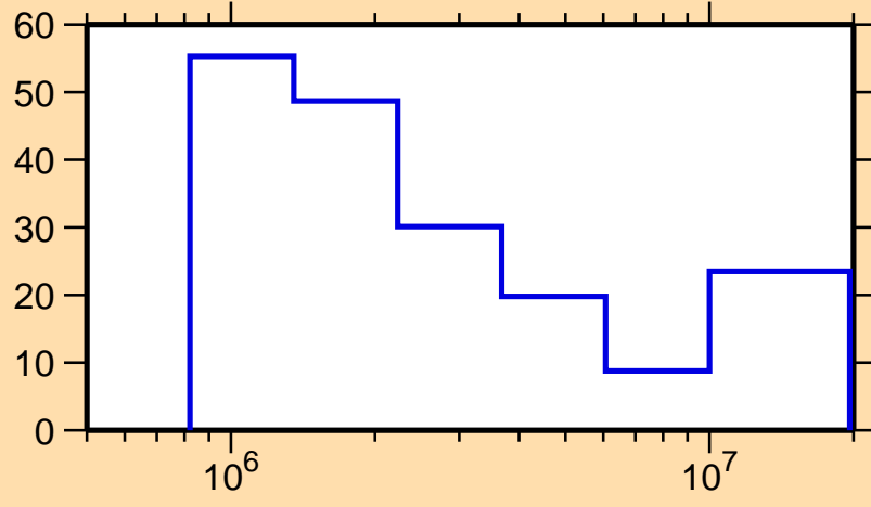
\Delta\sigma/\sigma vs. E for ^{163}\text{Yb}(n,n\text{cont.})
