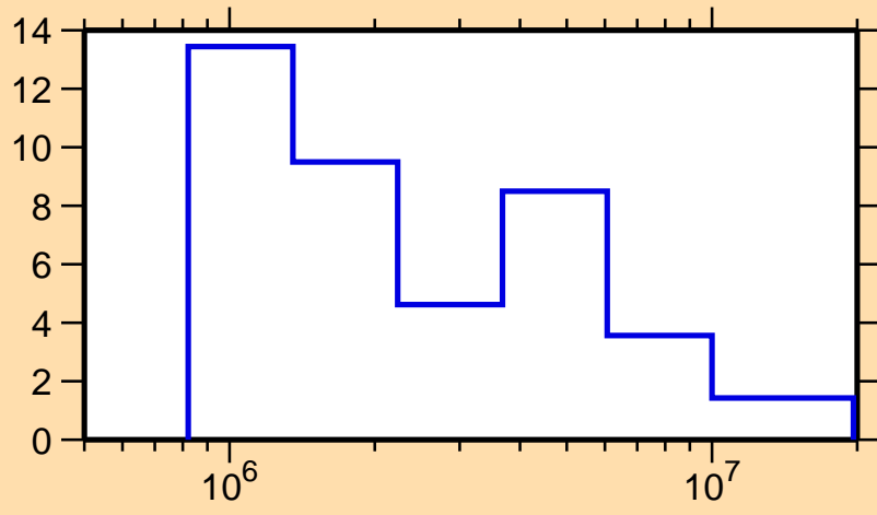
\Delta\sigma/\sigma vs. E for ^{163}\text{Yb}(n, \text{tot.})
