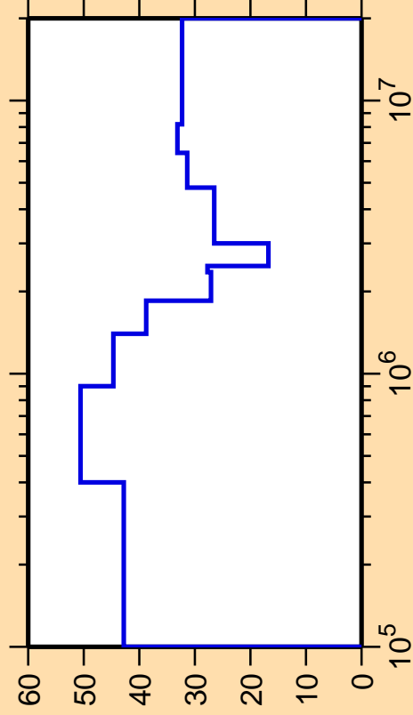
\Delta\sigma/\sigma vs. E for ^{163}\text{Yb}(n,n_4)
