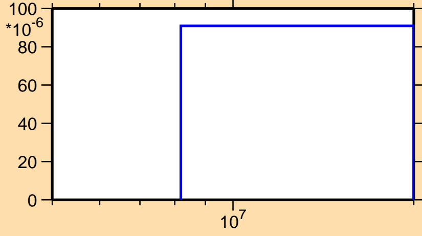
\sigma vs. E for ^{163}\text{Yb}(n,t)
