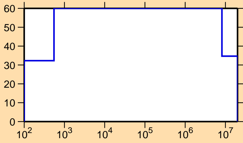
\Delta\sigma/\sigma vs. E for ^{163}\text{Yb}(n,p)
