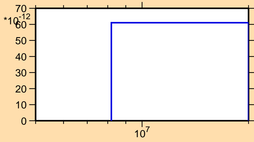
\sigma vs. E for ^{163}\text{Yb}(n,\text{pd})
