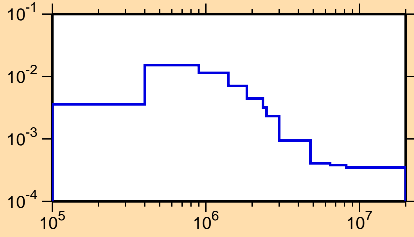
\sigma vs. E for ^{163}\text{Yb}(n,n_4)
