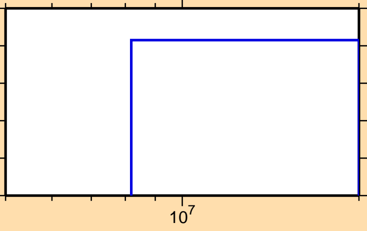
\sigma vs. E for ^{163}\text{Yb}(n,\text{He}3)
