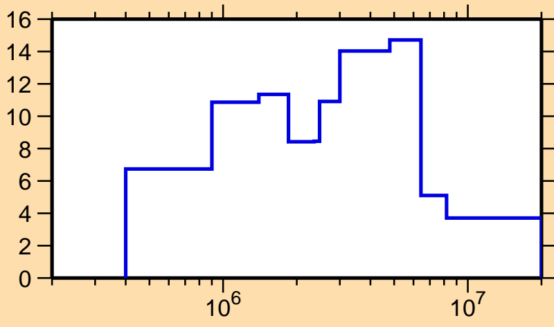
\Delta\sigma/\sigma vs. E for ^{163}\text{Yb}(n, el.)
