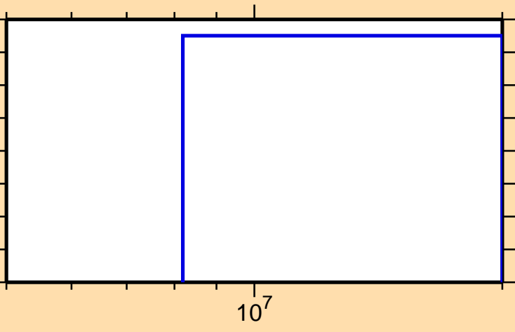
\sigma vs. E for ^{163}\text{Yb}(n,\text{nd})
