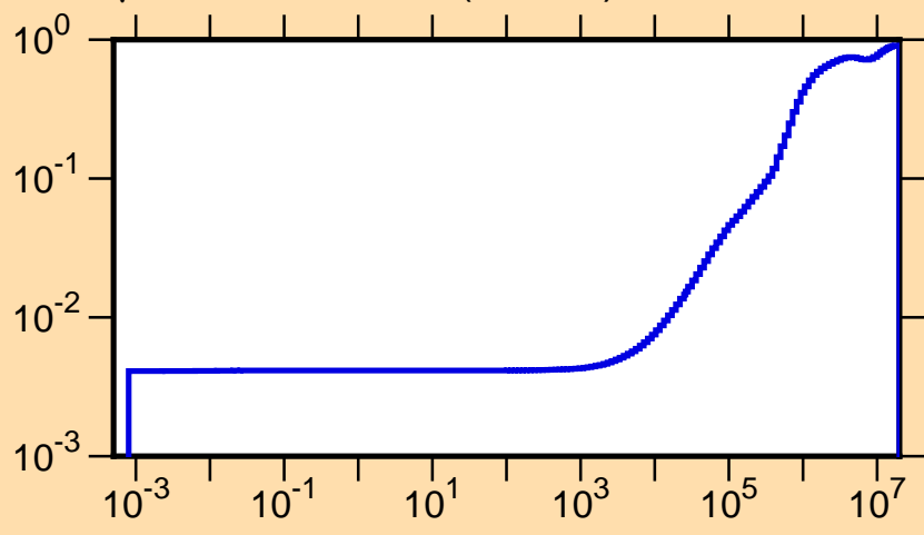
\mu vs. E for ^{164}\text{Yb}(\text{mt251})
