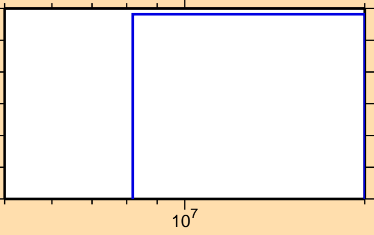
\sigma vs. E for ^{164}\text{Yb}(n,\text{He3})
