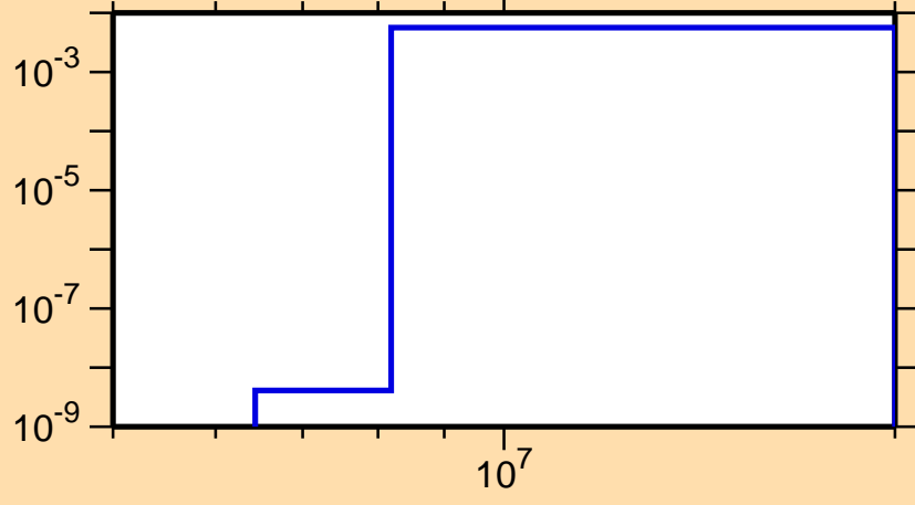
\sigma vs. E for ^{164}\text{Yb}(n,np)
