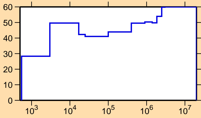
\Delta\sigma/\sigma vs. E for ^{164}\text{Yb}(n,\gamma)
