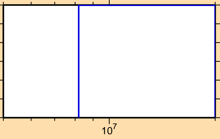
\sigma vs. E for ^{164}\text{Yb}(n,\text{nd})
