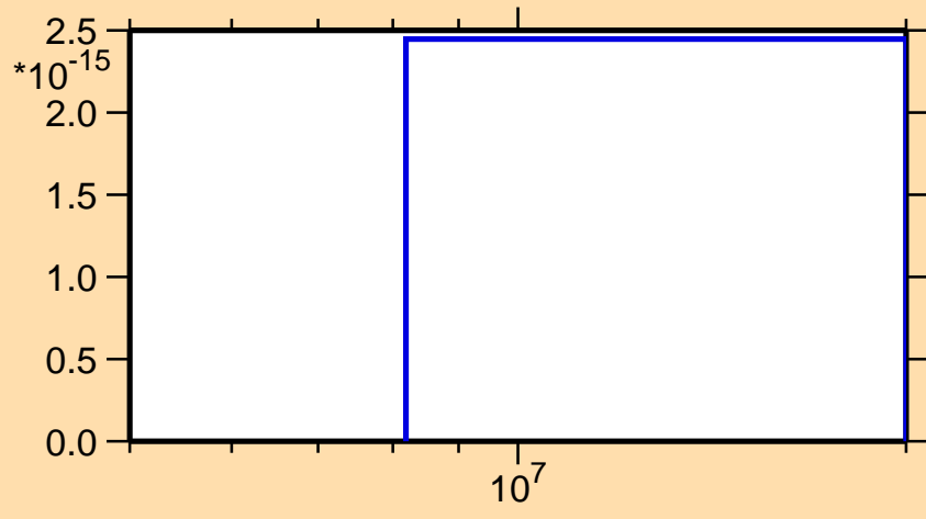
\sigma vs. E for ^{164}\text{Yb}(n,\text{pt})
