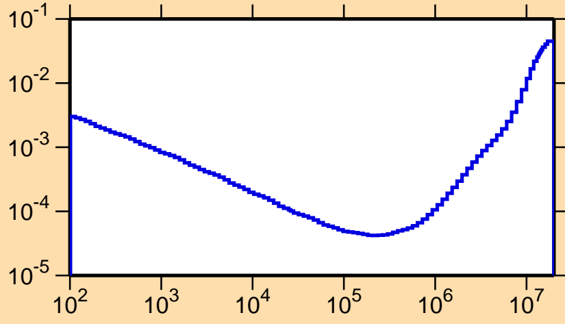
\sigma vs. E for ^{165}\text{Yb}(n,p)
