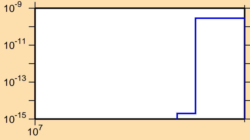
\sigma vs. E for ^{165}\text{Yb}(n,nt)
