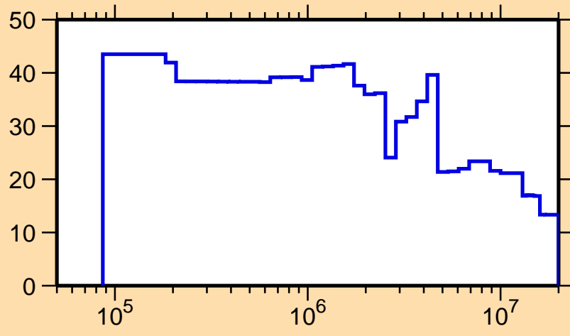
\Delta\sigma/\sigma vs. E for ^{165}\text{Yb}(n,n_1)
