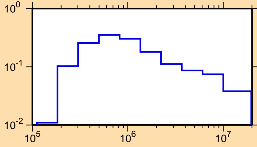
\sigma vs. E for ^{165}\text{Yb}(n,n_4)
