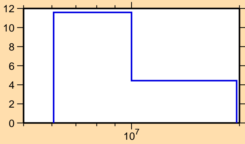
\Delta\sigma/\sigma vs. E for ^{165}\text{Yb}(n, 2n)
