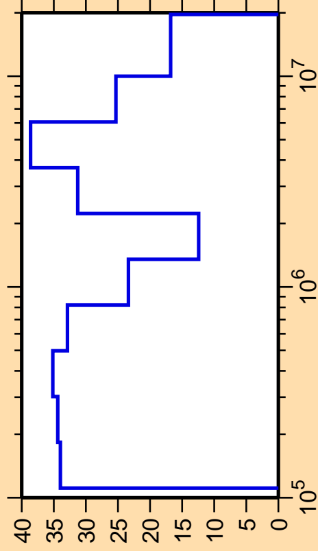
\Delta\sigma/\sigma vs. E for ^{165}\text{Yb}(n,n_4)
