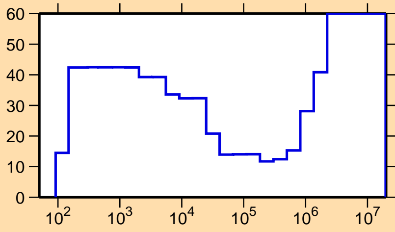
\Delta\sigma/\sigma vs. E for ^{165}\text{Yb}(n,\gamma)
