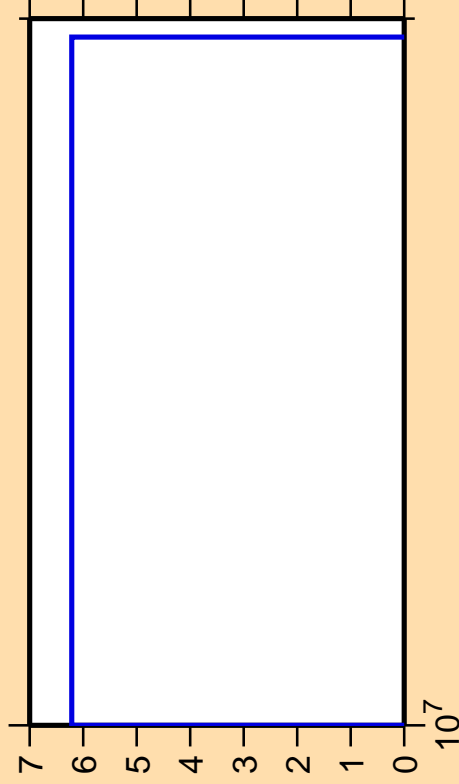
\Delta\sigma/\sigma vs. E for ^{165}\text{Yb}(\text{mt117})
