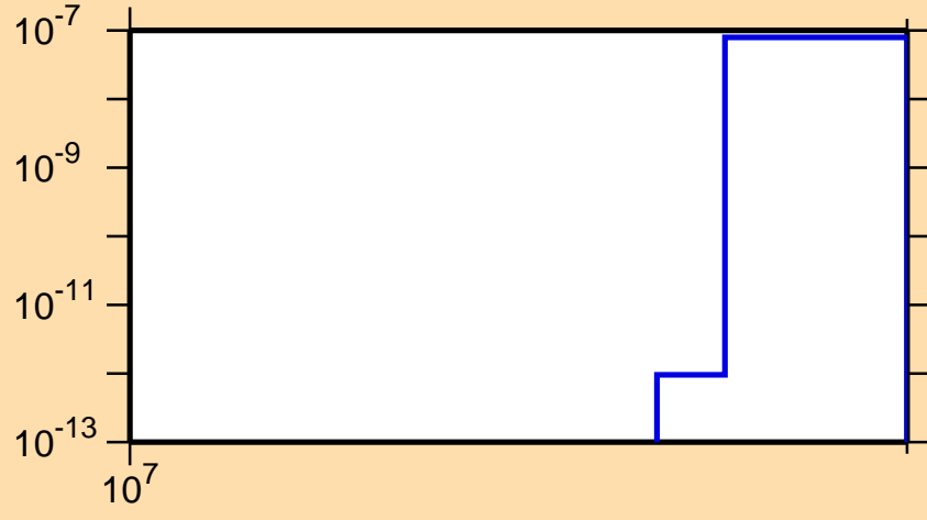
\sigma vs. E for ^{166}\text{Yb}(n,2np)
