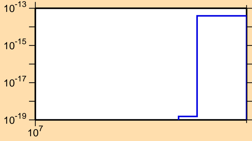
\sigma vs. E for ^{166}\text{Yb}(n,3n\alpha)
