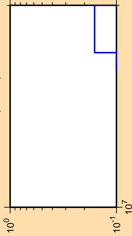
\Delta\sigma/\sigma vs. E for ^{166}\text{Yb}(n,3n\alpha)
