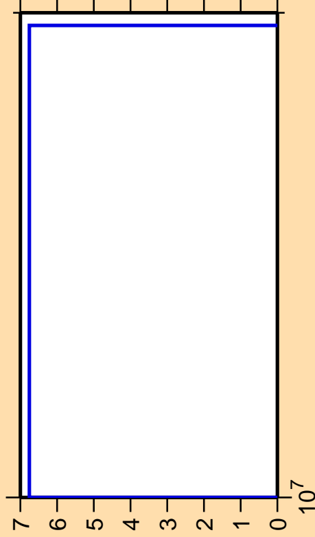
\Delta\sigma/\sigma vs. E for ^{166}\text{Yb}(\text{mt117})
