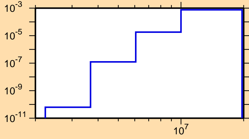
\sigma vs. E for ^{166}\text{Yb}(n,n\alpha)
