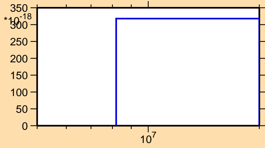
\sigma vs. E for ^{166}\text{Yb}(n,3n\alpha)
