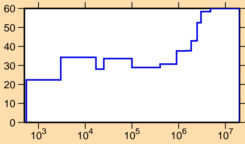
\Delta\sigma/\sigma vs. E for ^{166}\text{Yb}(n,\gamma)
