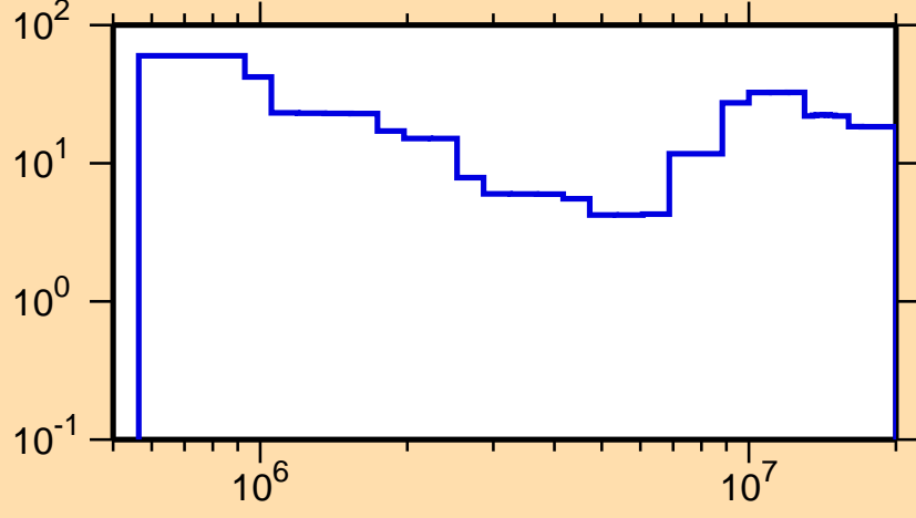
\Delta\sigma/\sigma vs. E for ^{167}\text{Yb}(n,n\text{cont.})
