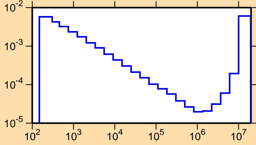
\sigma vs. E for ^{167}\text{Yb}(n,\alpha)
