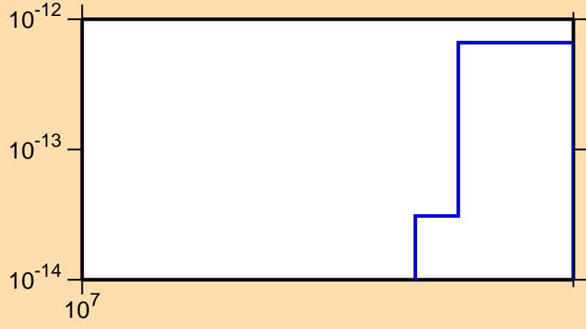
\sigma vs. E for ^{169}\text{Yb} (mt 45)
