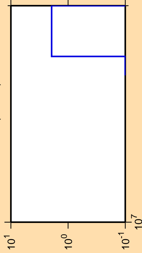
\Delta\sigma/\sigma vs. E for ^{169}\text{Yb} (mt 34)
