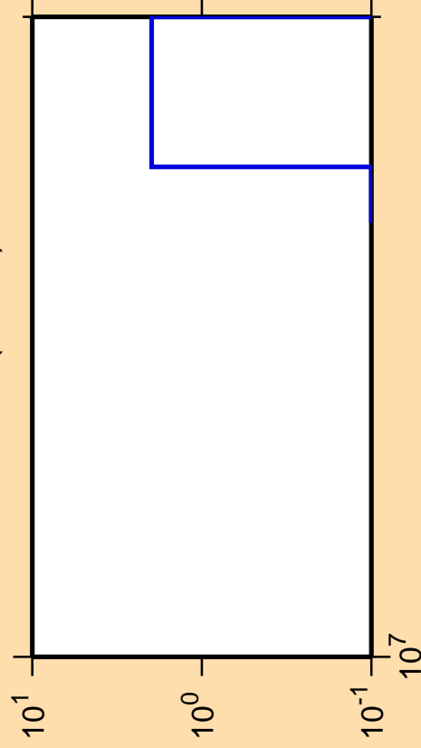
\Delta\sigma/\sigma vs. E for ^{169}\text{Yb} (mt 45)
