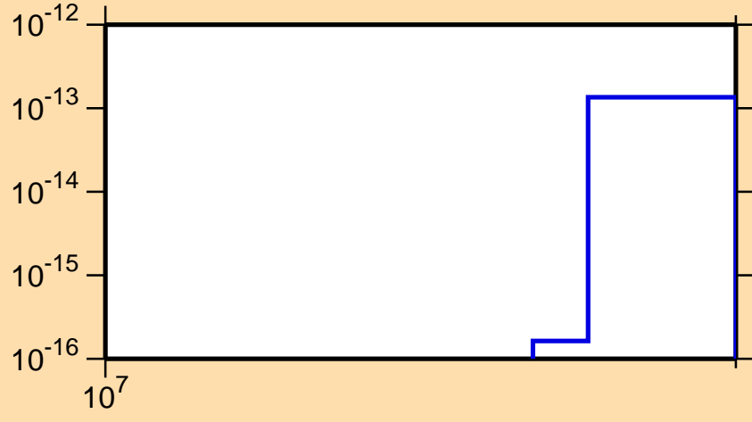
\sigma vs. E for ^{169}\text{Yb}(n,\text{pt})
