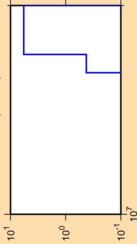
\Delta\sigma/\sigma vs. E for ^{169}\text{Yb}(\text{mt117})
