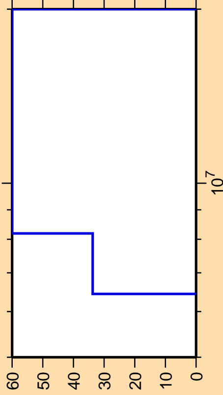
\Delta\sigma/\sigma vs. E for ^{169}\text{Yb}(n,n\text{cont.})
