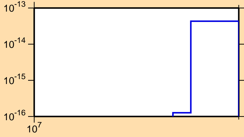
\sigma vs. E for ^{169}\text{Yb}(n,\text{pd})
