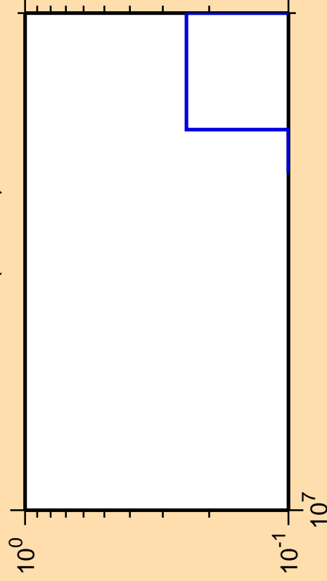
\Delta\sigma/\sigma vs. E for ^{169}\text{Yb}(n,3n\alpha)
