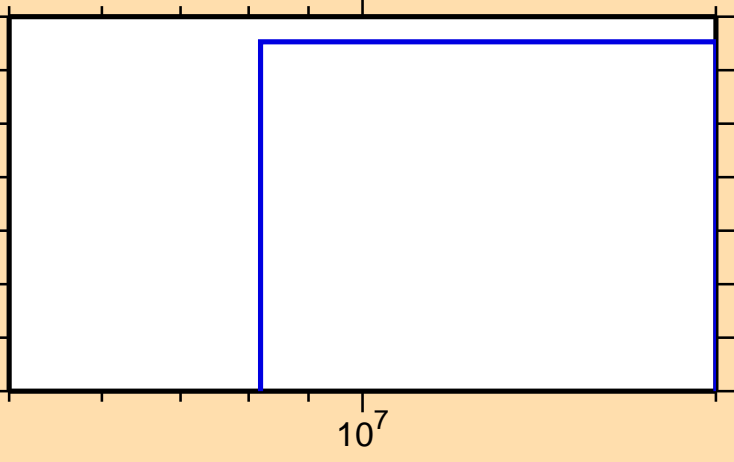
\sigma vs. E for ^{169}\text{Yb}(\text{mt117})
