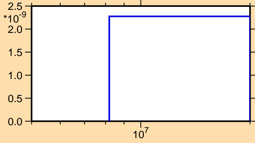
\sigma vs. E for ^{169}\text{Yb}(n,p\alpha)
