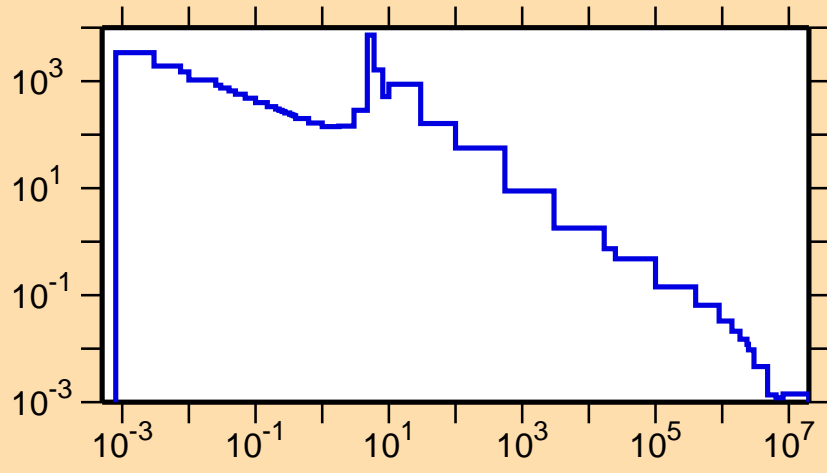
\sigma vs. E for ^{169}\text{Yb}(n,\gamma)
