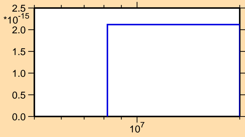
\sigma vs. E for ^{169}\text{Yb}(n,3n\alpha)
