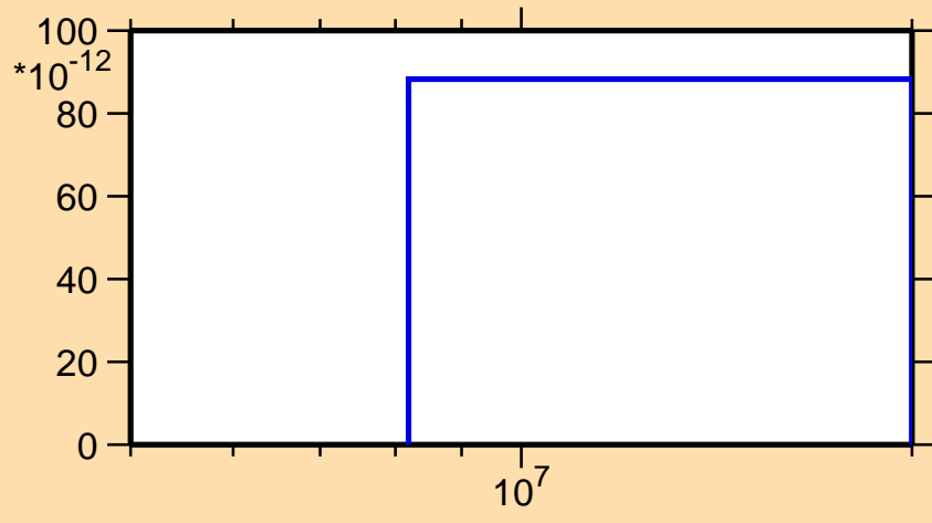
\sigma vs. E for ^{169}\text{Yb}(n,nt)
