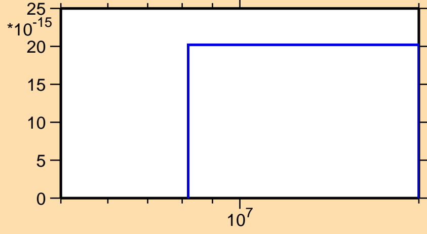
\sigma vs. E for ^{169}\text{Yb} (mt 45)
