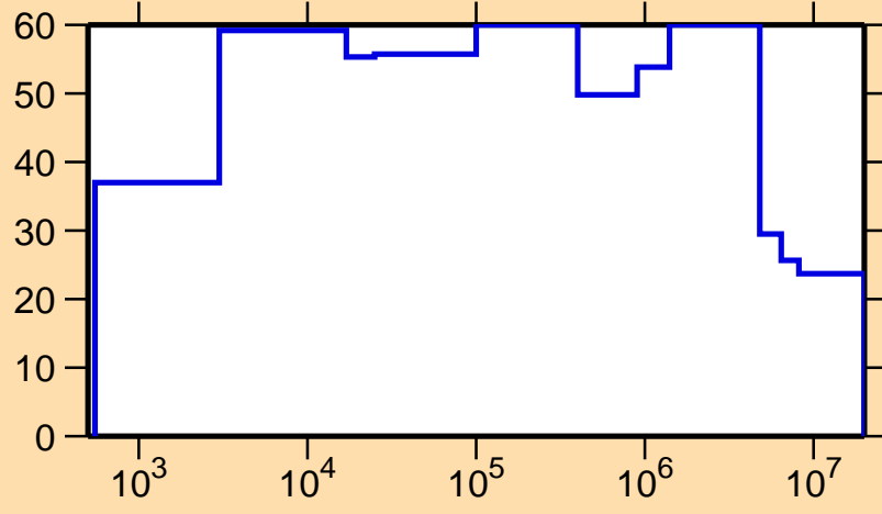
\Delta\sigma/\sigma vs. E for ^{169}\text{Yb}(n,p)
