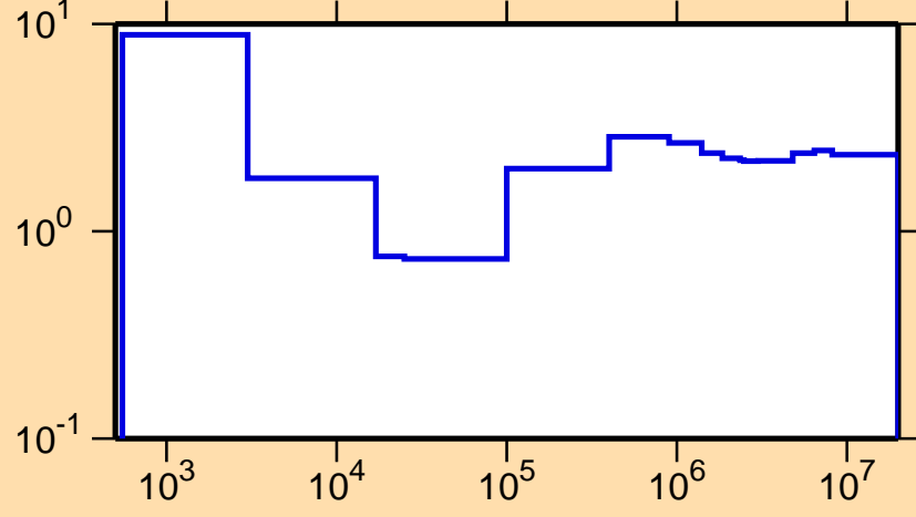
\sigma vs. E for ^{169}\text{Yb}(n,\text{nonel.})
