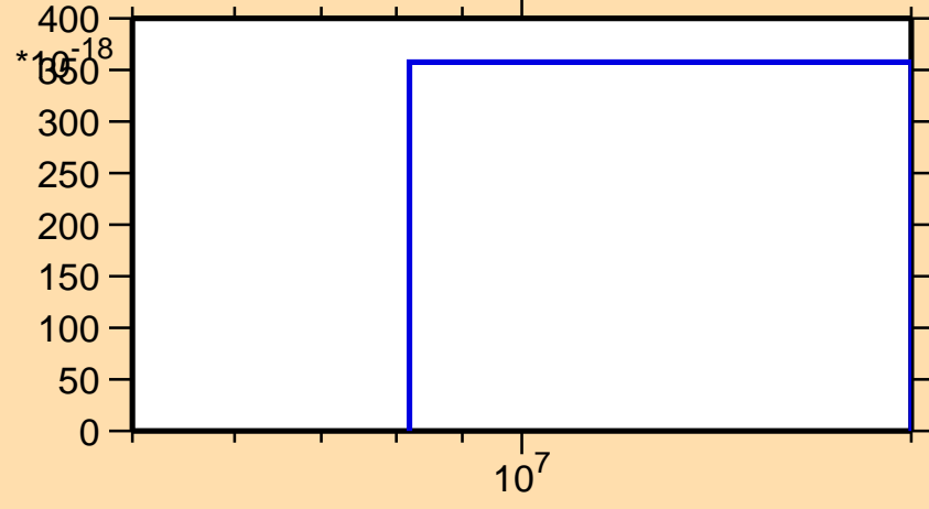
\sigma vs. E for ^{169}\text{Yb}(n,\text{pd})
