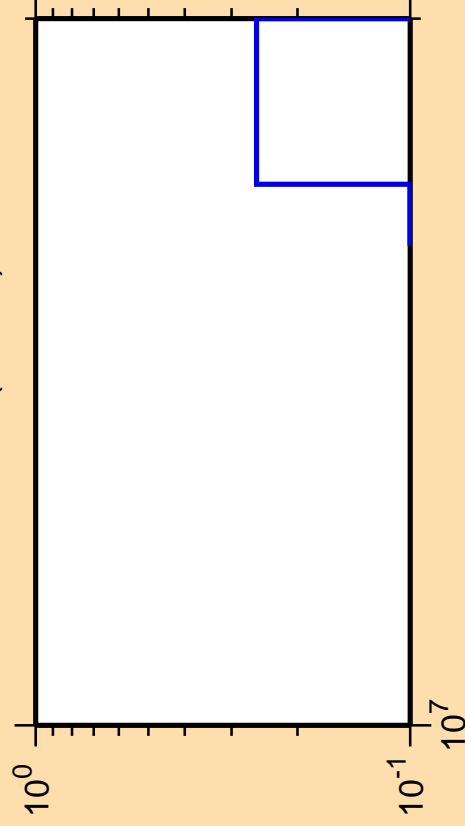
\Delta\sigma/\sigma vs. E for ^{170}\text{Yb}(n,3n\alpha)
