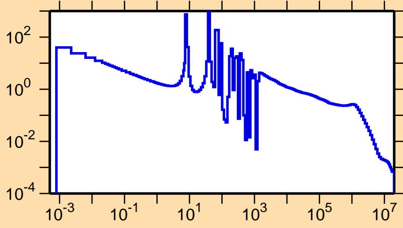
\sigma vs. E for ^{170}\text{Yb}(n,\gamma)
