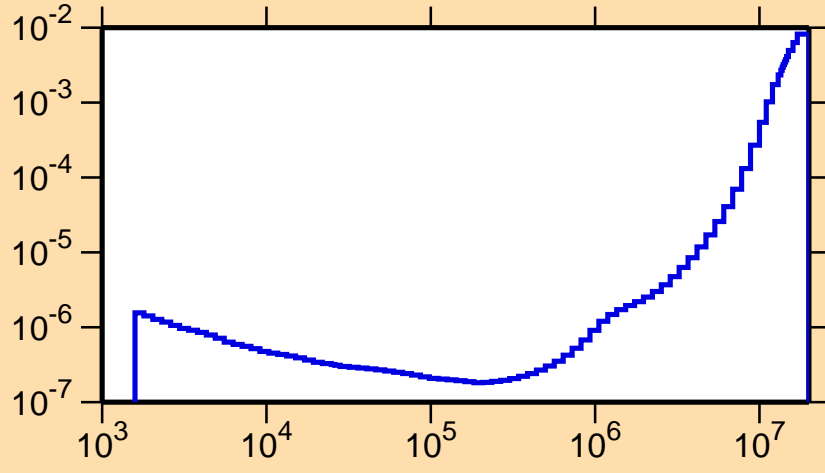
\sigma vs. E for ^{170}\text{Yb}(n,\alpha)
