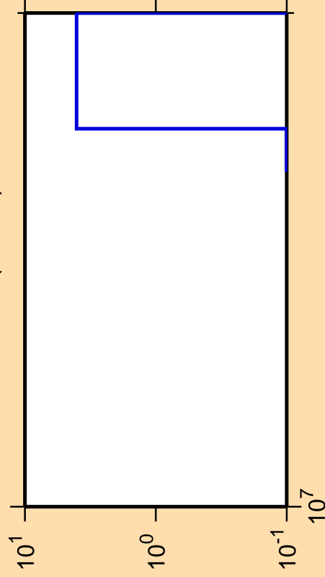
\Delta\sigma/\sigma vs. E for ^{170}\text{Yb} (mt 45)
