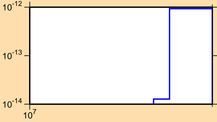
\sigma vs. E for ^{170}\text{Yb} (mt 45)
