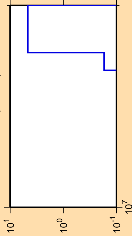
\Delta\sigma/\sigma vs. E for ^{170}\text{Yb}(\text{mt117})
