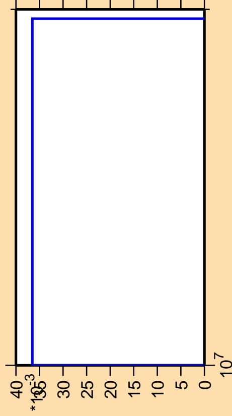
\Delta\sigma/\sigma vs. E for ^{170}\text{Yb} (mt 45)
