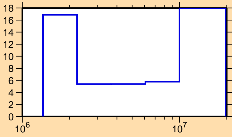
\Delta\sigma/\sigma vs. E for ^{170}\text{Yb}(n,n\text{cont.})
