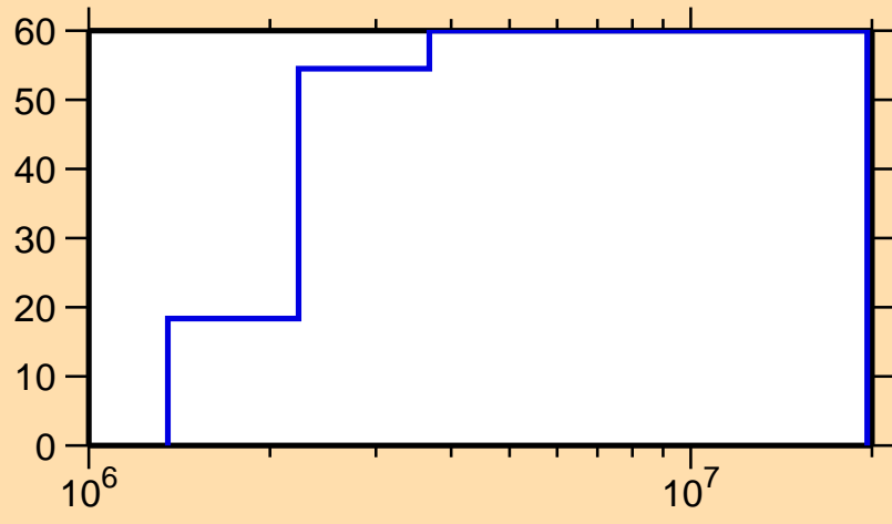
\Delta\sigma/\sigma vs. E for ^{170}\text{Yb}(n,\gamma)
