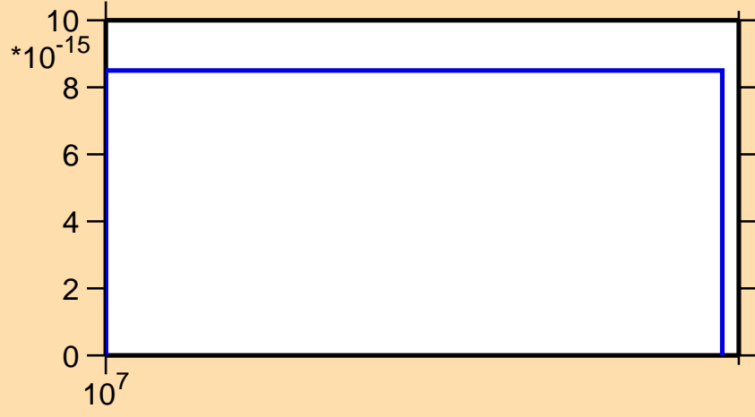
\sigma vs. E for ^{170}\text{Yb} (mt 45)
