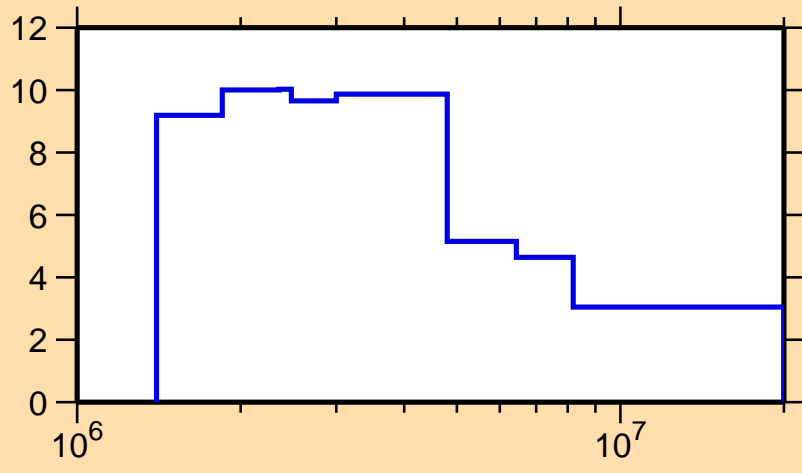
\Delta\sigma/\sigma vs. E for ^{170}\text{Yb}(n, el.)
