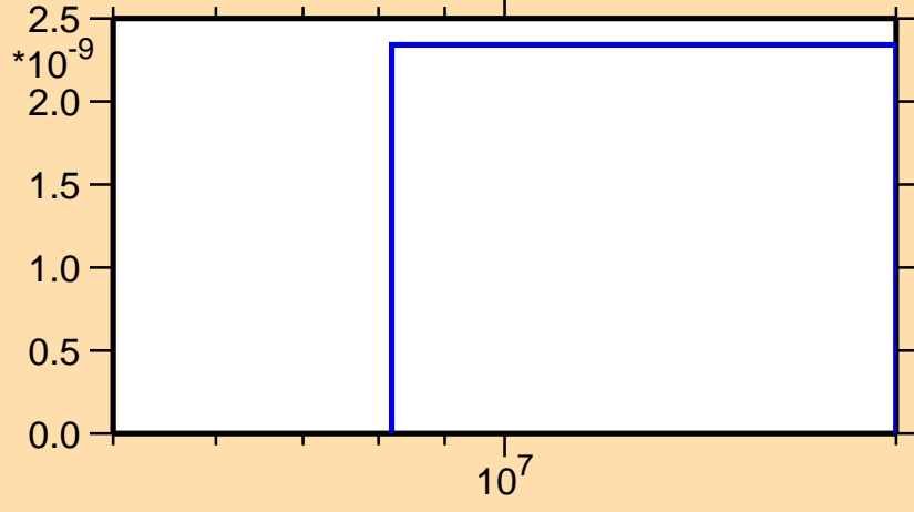
\sigma vs. E for ^{170}\text{Yb}(n,\text{nd})
