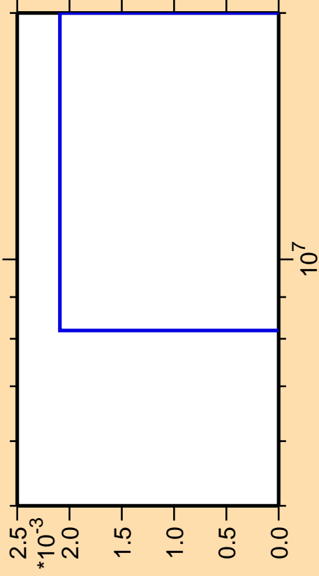
\Delta\sigma/\sigma vs. E for ^{170}\text{Yb}(n,3n\alpha)
