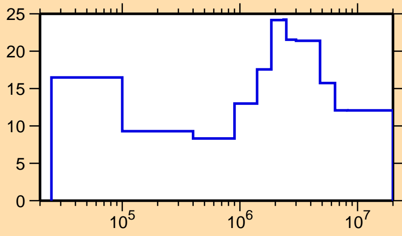
\Delta\sigma/\sigma vs. E for ^{170}\text{Yb}(n,n_1)
