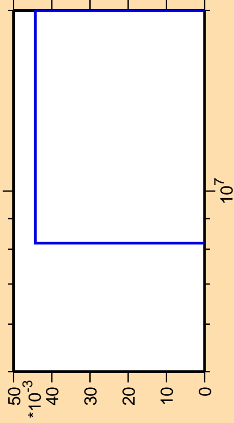
\Delta\sigma/\sigma vs. E for ^{170}\text{Yb}(\text{mt117})
