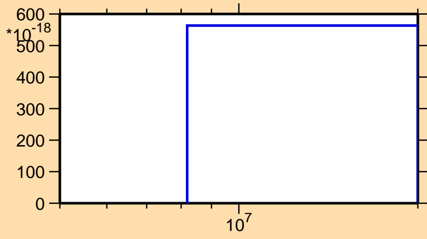
\sigma vs. E for ^{170}\text{Yb}(n,3n\alpha)
