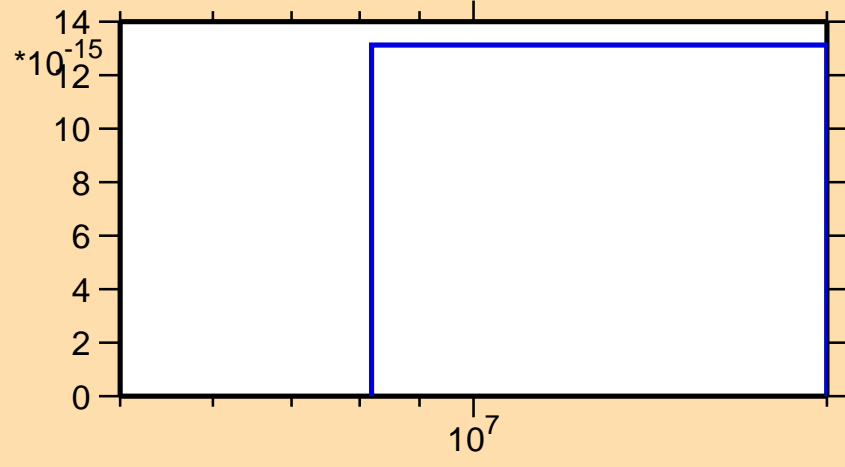
\sigma vs. E for ^{170}\text{Yb}(\text{mt117})
