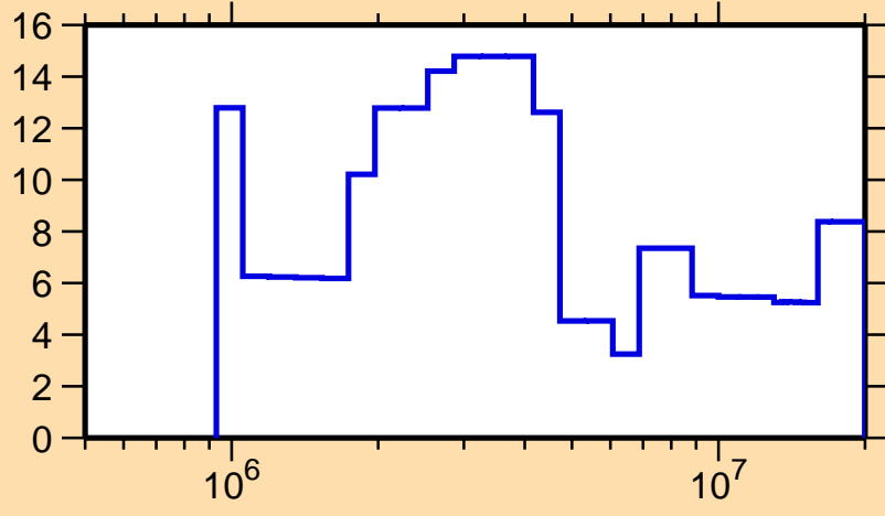
\Delta\sigma/\sigma vs. E for ^{171}\text{Yb}(n,el.)
