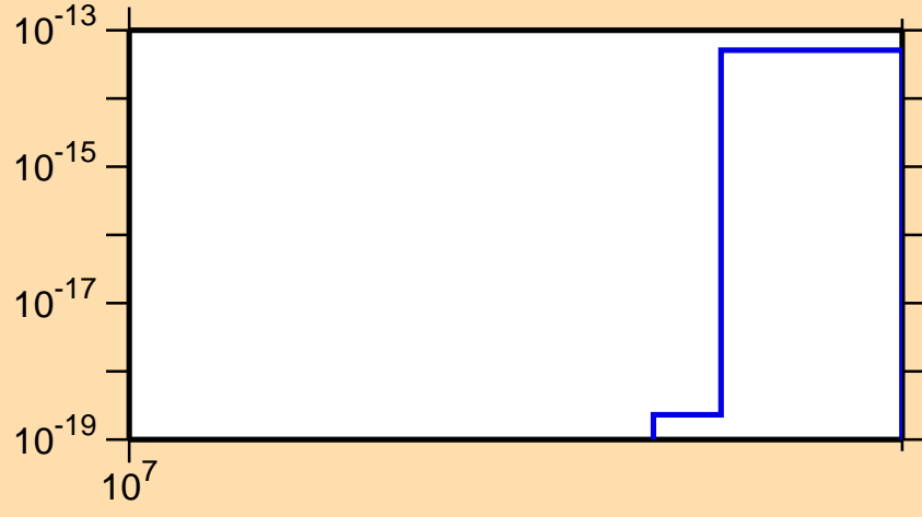
\sigma vs. E for ^{171}\text{Yb}(n,3n\alpha)
