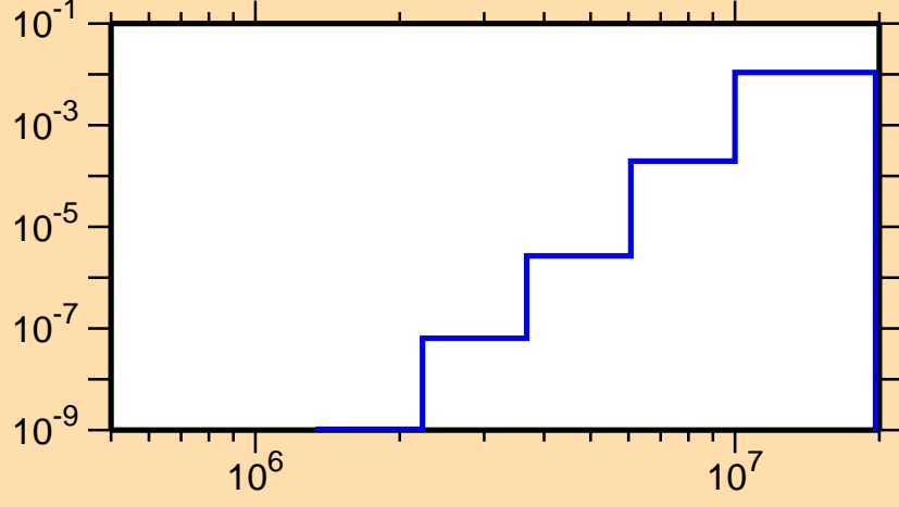
\sigma vs. E for ^{171}\text{Yb}(n,p)
