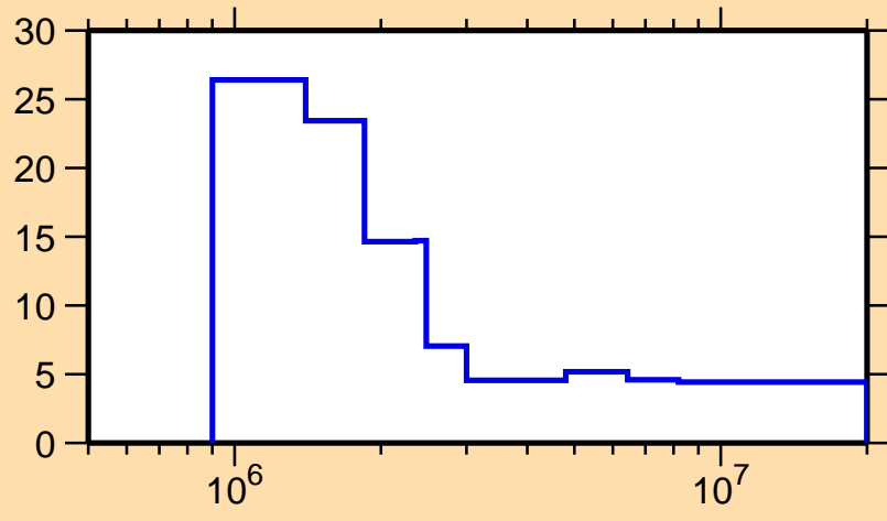
\Delta\sigma/\sigma vs. E for ^{171}\text{Yb}(n,\text{nonel.})
