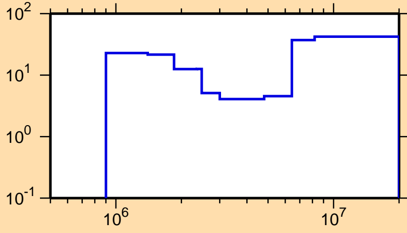
\Delta\sigma/\sigma vs. E for ^{171}\text{Yb}(n,n\text{cont.})
