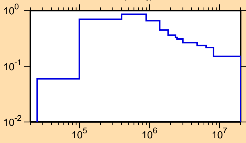
\sigma vs. E for ^{171}\text{Yb}(n,n_1)
