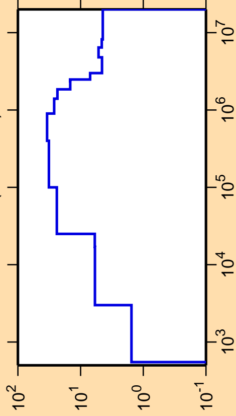
\Delta\sigma/\sigma vs. E for ^{171}\text{Yb}(n,\text{nonel.})
