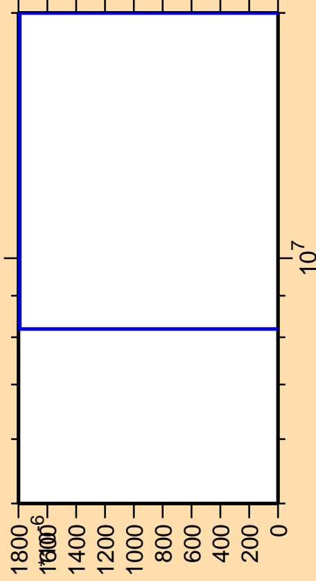
\Delta\sigma/\sigma vs. E for ^{171}\text{Yb}(n,3n\alpha)
