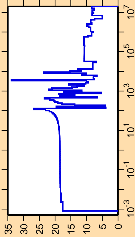
\Delta\sigma/\sigma vs. E for ^{172}\text{Yb}(n,\text{el.})
