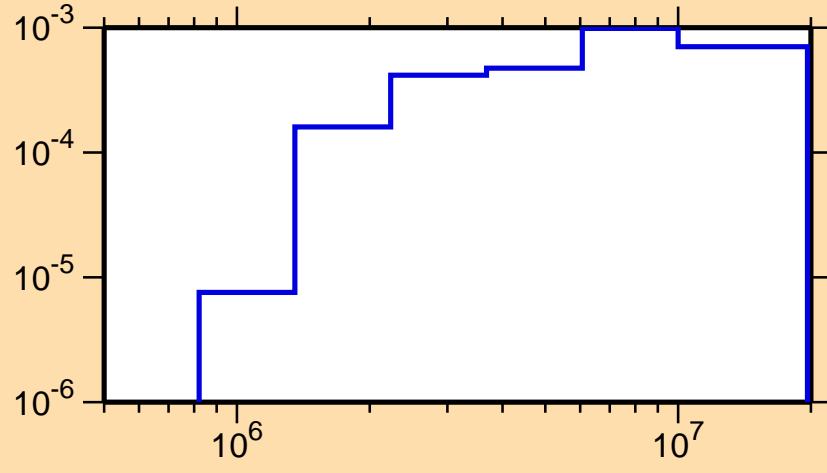
\sigma vs. E for ^{172}\text{Yb}(n,n_4)
