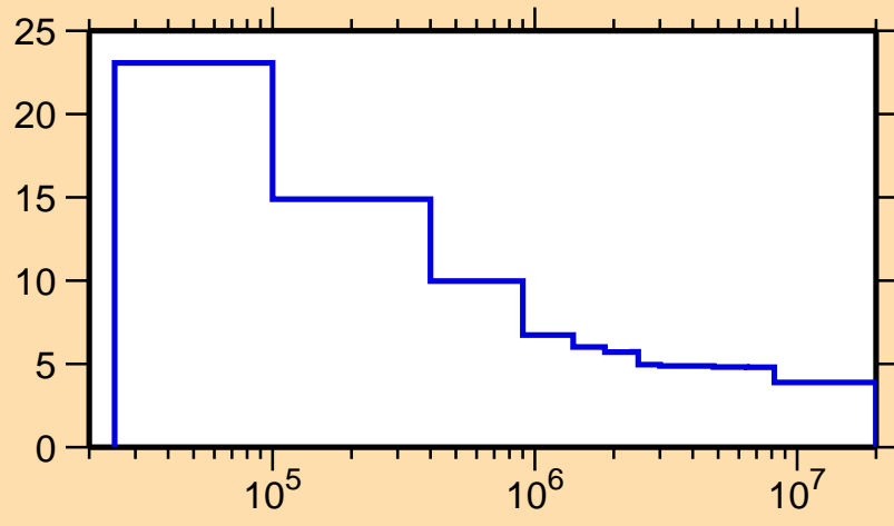
\Delta\sigma/\sigma vs. E for ^{172}\text{Yb}(n,\text{nonel.})
