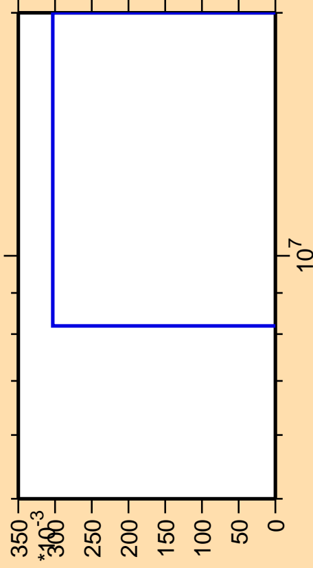
\Delta\sigma/\sigma vs. E for ^{172}\text{Yb}(n,p\alpha)
