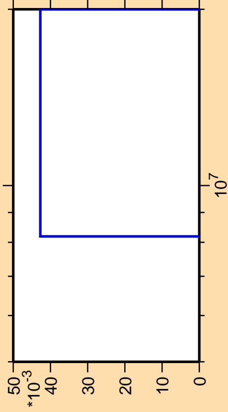
\Delta\sigma/\sigma vs. E for ^{172}\text{Yb}(n,3n\alpha)
