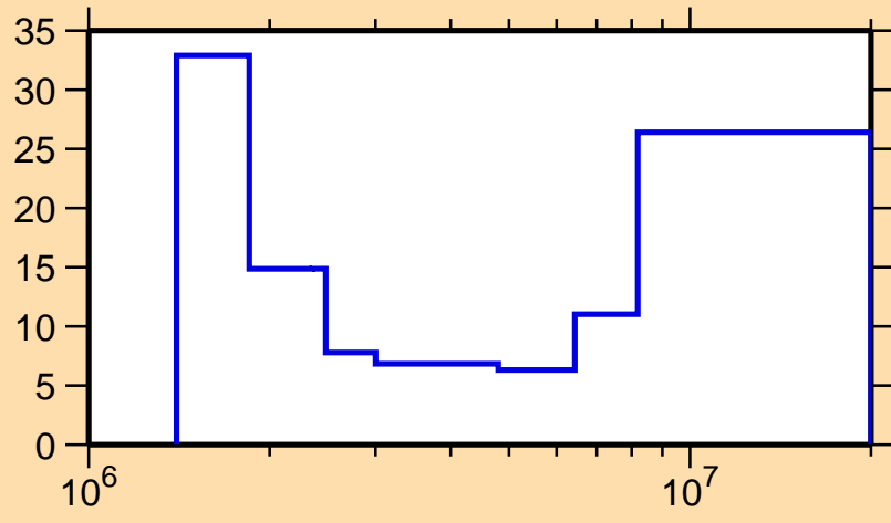
\Delta\sigma/\sigma vs. E for ^{172}\text{Yb}(n,n\text{cont.})
