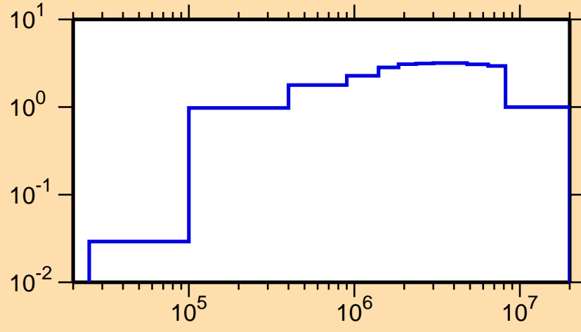
\sigma vs. E for ^{172}\text{Yb}(n,\text{inel.})
