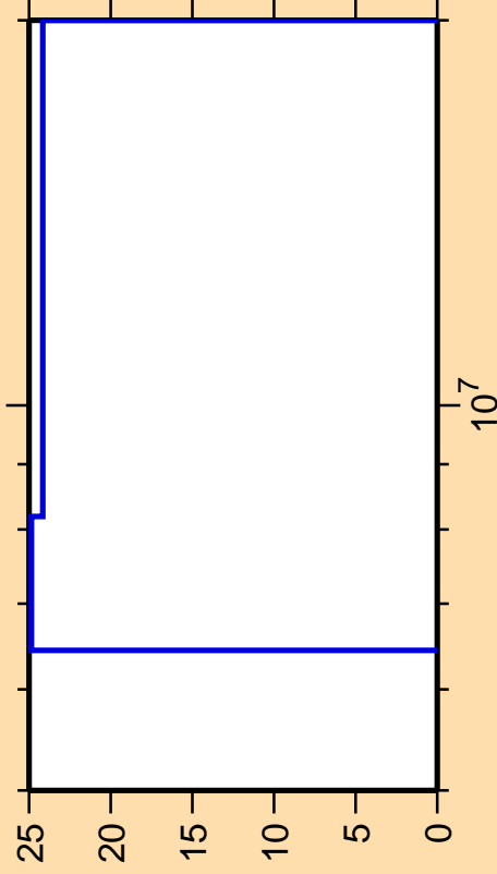
\Delta\sigma/\sigma vs. E for ^{172}\text{Yb}(n,n_1)
