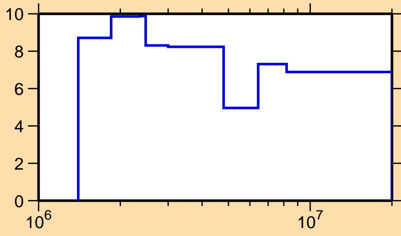
\Delta\sigma/\sigma vs. E for ^{172}\text{Yb}(n, el.)
