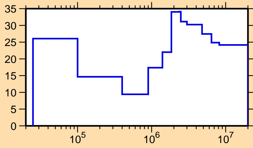
\Delta\sigma/\sigma vs. E for ^{172}\text{Yb}(n,n_1)
