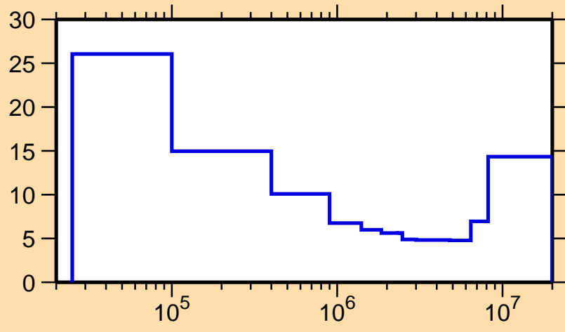
\Delta\sigma/\sigma vs. E for ^{172}\text{Yb}(n,\text{inel.})
