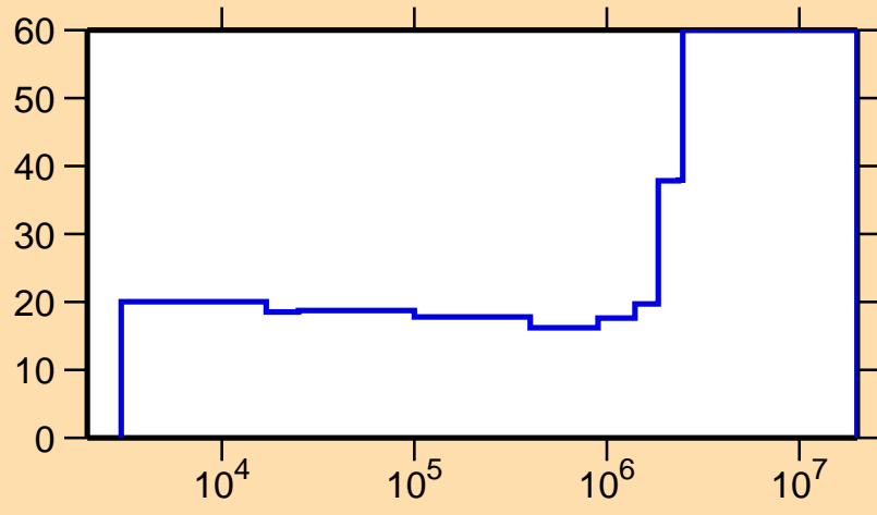
\Delta\sigma/\sigma vs. E for ^{172}\text{Yb}(n,\gamma)
