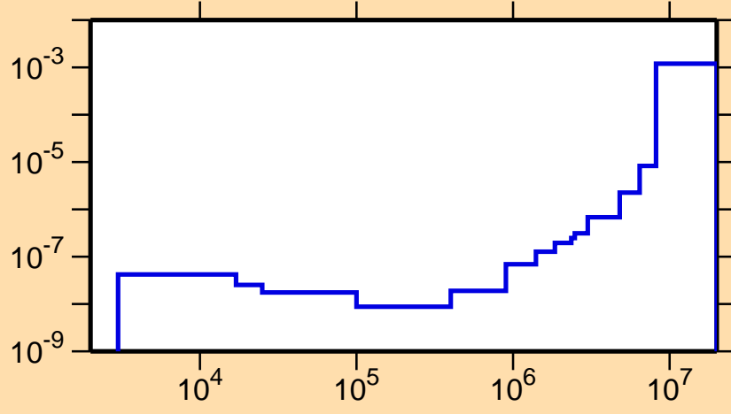
\sigma vs. E for ^{172}\text{Yb}(n,\alpha)
