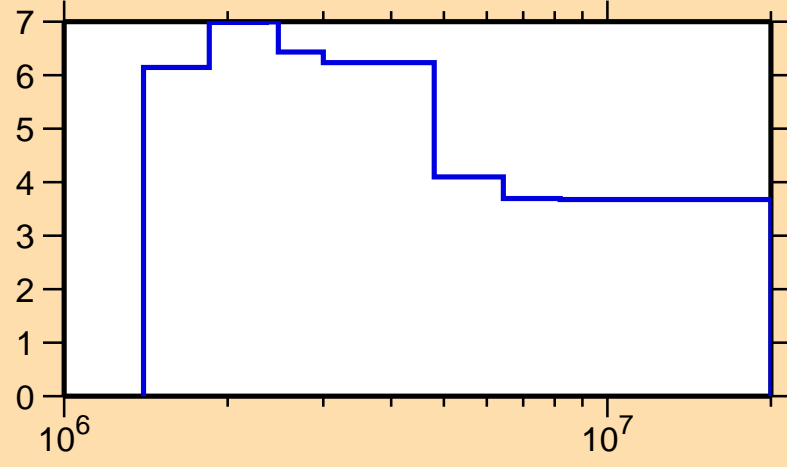
\Delta\sigma/\sigma vs. E for ^{172}\text{Yb}(n, \text{tot.})
