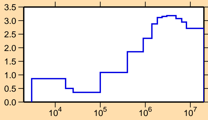
\sigma vs. E for ^{172}\text{Yb}(n,\text{nonel.})
