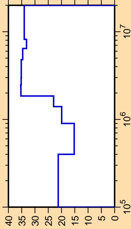
\Delta\sigma/\sigma vs. E for ^{172}\text{Yb}(n,n_2)
