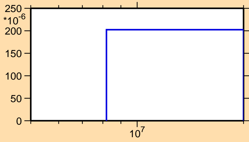
\sigma vs. E for ^{172}\text{Yb}(n,np)
