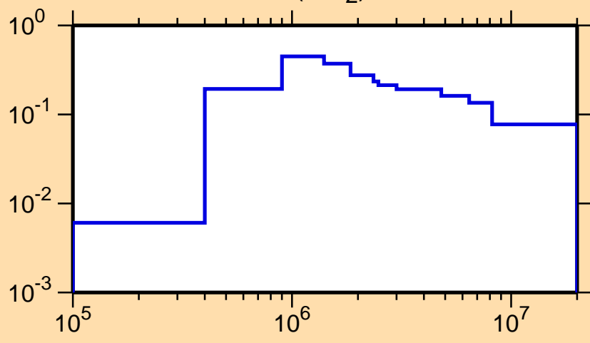
\sigma vs. E for ^{172}\text{Yb}(n,n_2)
