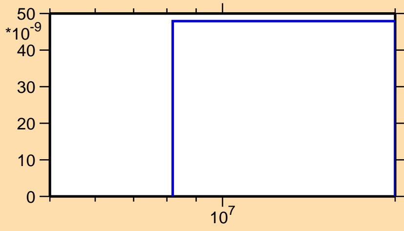
\sigma vs. E for ^{172}\text{Yb}(n,2n\alpha)
