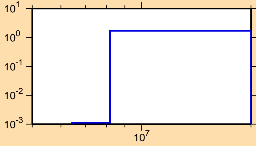
\sigma vs. E for ^{172}\text{Yb}(n,2n)
