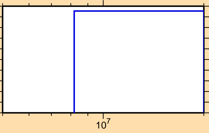
\sigma vs. E for ^{172}\text{Yb}(n,t)
