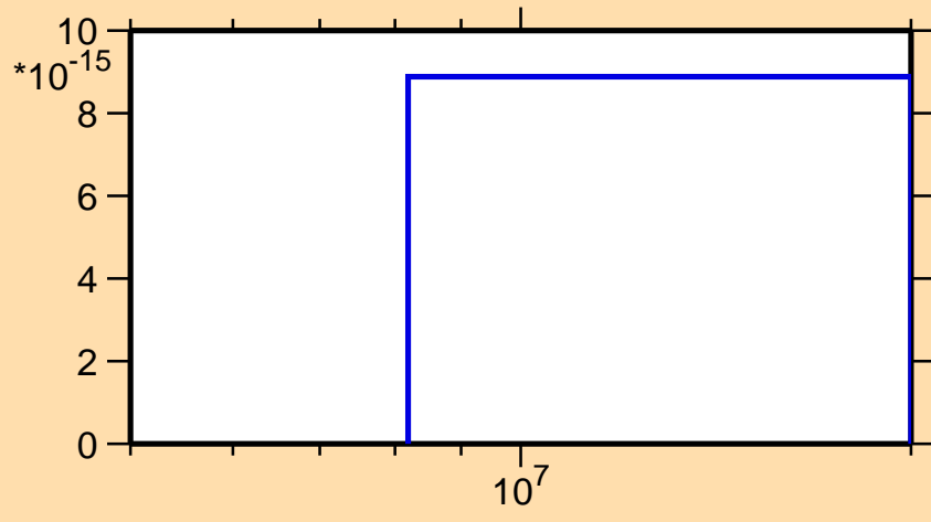
\sigma vs. E for ^{172}\text{Yb}(n,3n\alpha)
