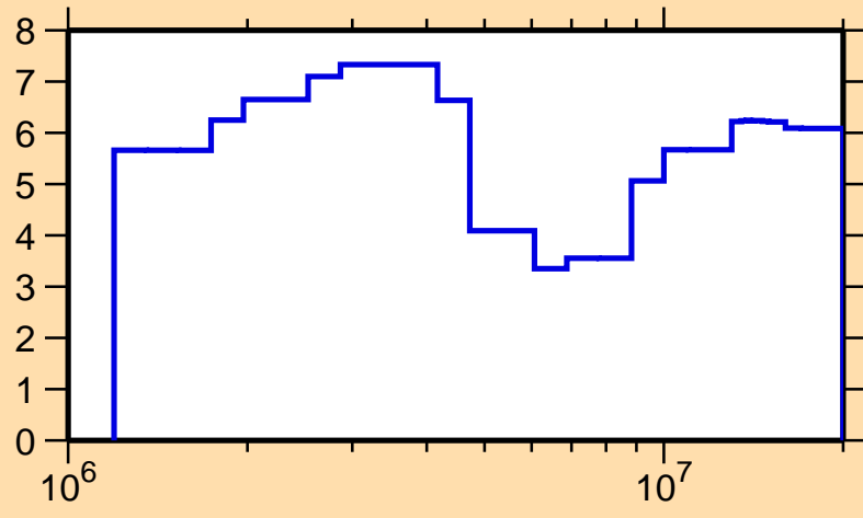
\Delta\sigma/\sigma vs. E for ^{173}\text{Yb}(n, el.)
