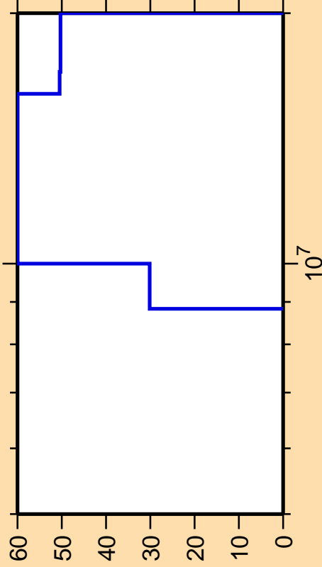
\Delta\sigma/\sigma vs. E for ^{173}\text{Yb}(n,np)
