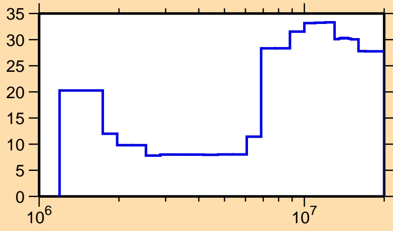
\Delta\sigma/\sigma vs. E for ^{173}\text{Yb}(n,n\text{cont.})
