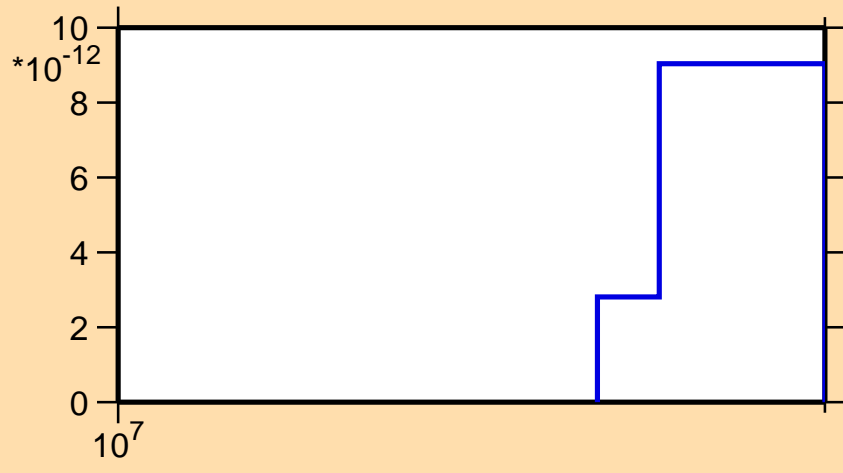
\sigma vs. E for ^{173}\text{Yb}(n,p\alpha)
