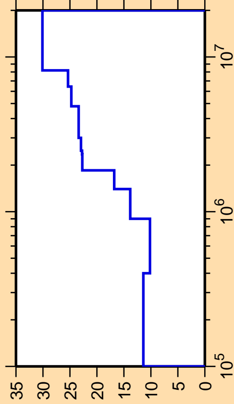
\Delta\sigma/\sigma vs. E for ^{173}\text{Yb}(n,n_2)
