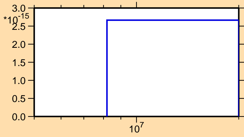
\sigma vs. E for ^{173}\text{Yb}(n,3n\alpha)
