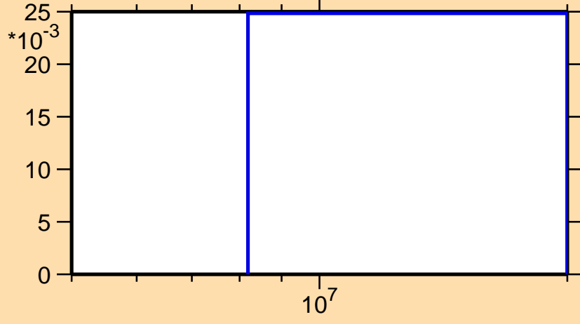
\sigma vs. E for ^{173}\text{Yb}(n,3n)
