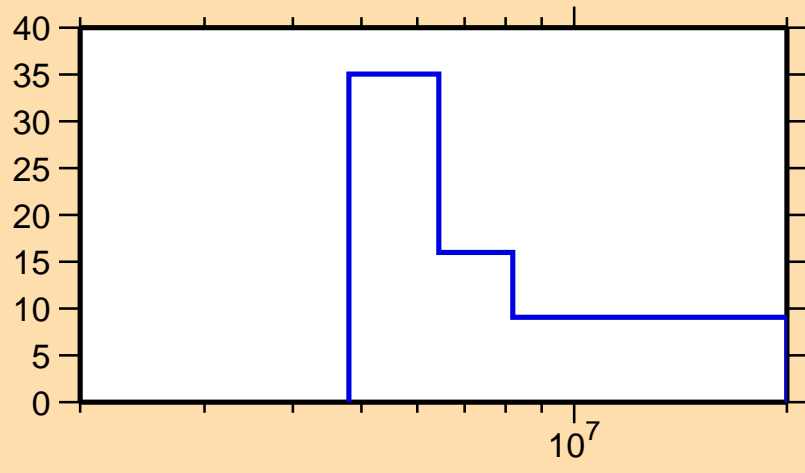
\Delta\sigma/\sigma vs. E for ^{173}\text{Yb}(n, 2n)
