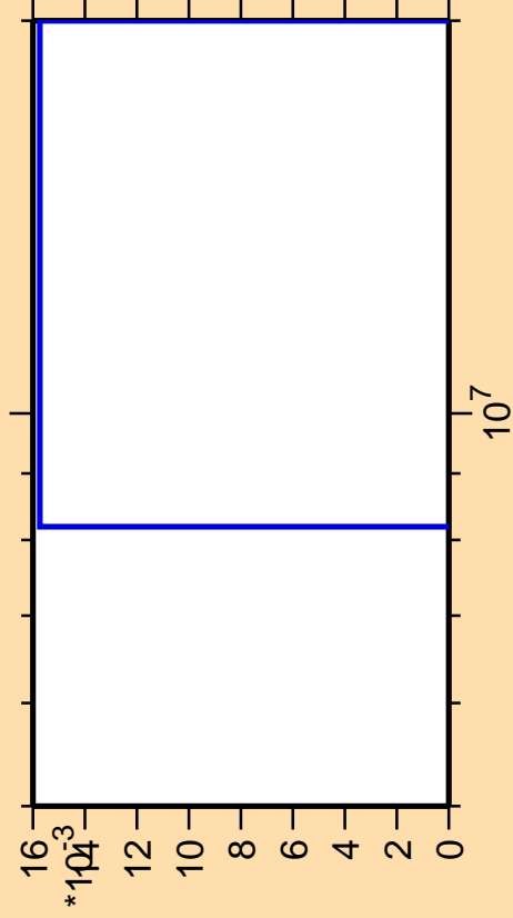
\Delta\sigma/\sigma vs. E for ^{173}\text{Yb}(n,3n\alpha)
