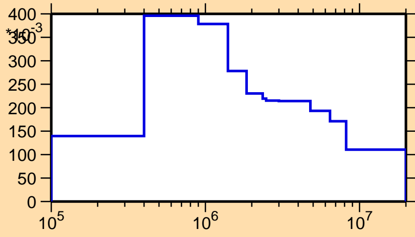
\sigma vs. E for ^{173}\text{Yb}(n,n_2)
