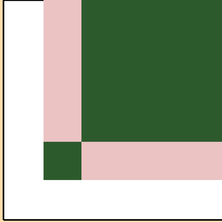
\sigma vs. E for ^{176}\text{Yb}(n,2n)
