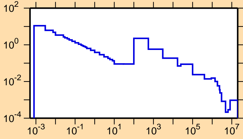
\sigma vs. E for ^{176}\text{Yb}(n,\gamma)
