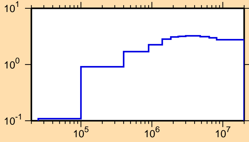
\sigma vs. E for ^{176}\text{Yb}(n,\text{nonel.})
