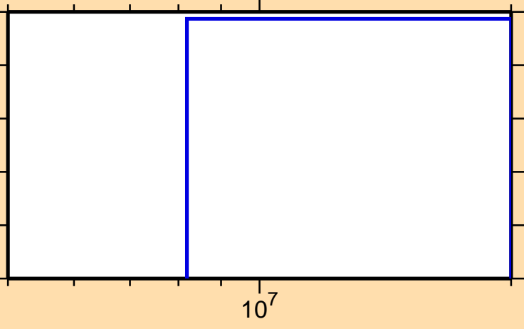
\sigma vs. E for ^{176}\text{Yb}(n,\text{nd})
