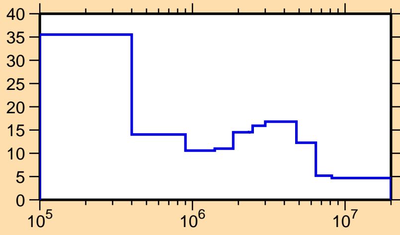
\Delta\sigma/\sigma vs. E for ^{177}\text{Yb}(n,\text{tot.})
