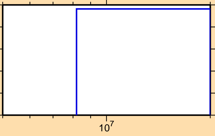
\sigma vs. E for ^{177}\text{Yb}(n,\text{nd})
