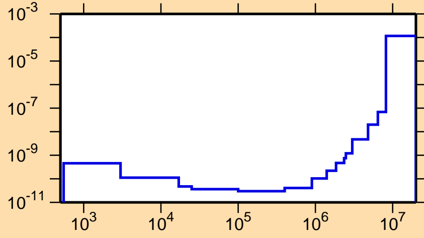
\sigma vs. E for ^{177}\text{Yb}(n,\alpha)
