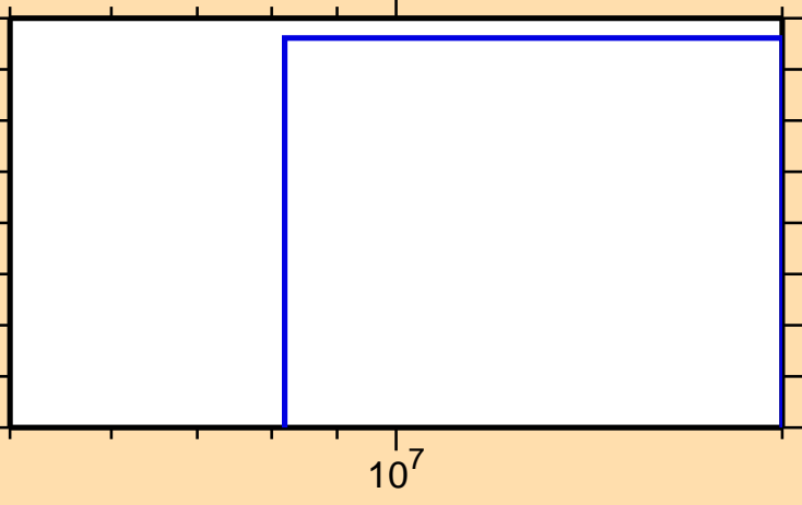
\sigma vs. E for ^{177}\text{Yb}(n,t)
