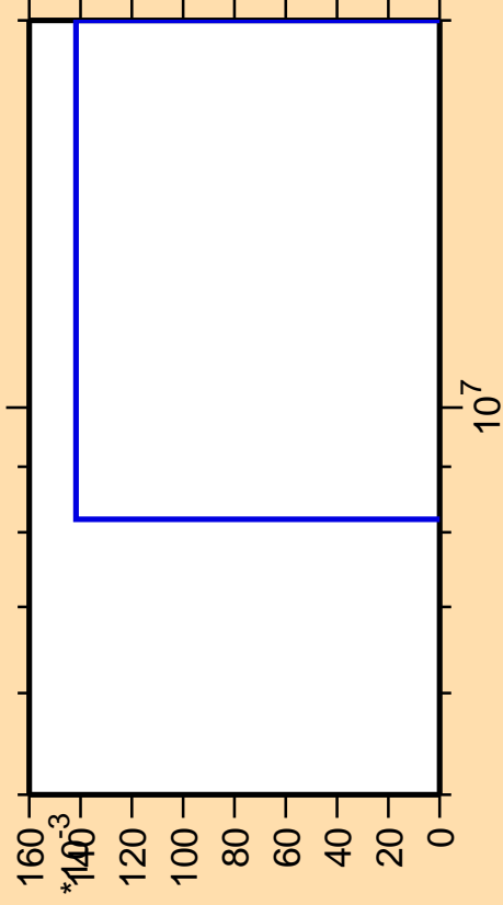
\Delta\sigma/\sigma vs. E for ^{177}\text{Yb}(n,3n\alpha)
