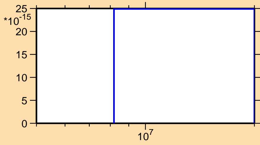
\sigma vs. E for ^{177}\text{Yb}(n,3n\alpha)
