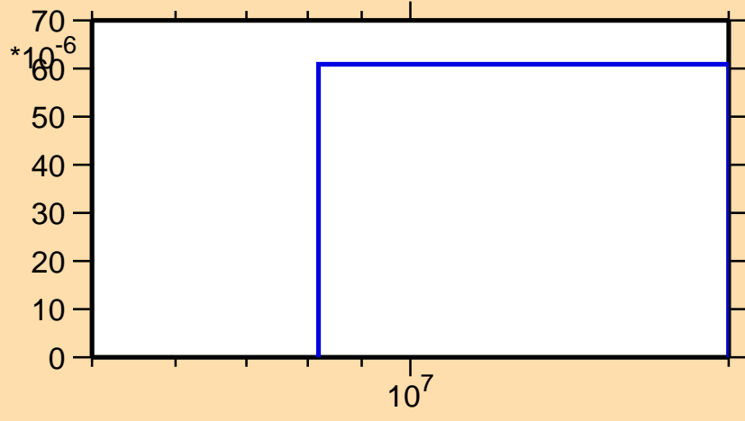
\sigma vs. E for ^{177}\text{Yb}(n,d)
